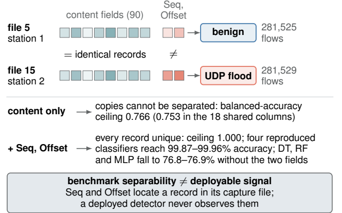
FIGURE 4. The label conflict in \mathcal{D}_B (schematic tiles). Identical flow records occur in two capture files, one per base station, labeled benign in one and UDP flood in the other, so no function of the record content can separate them. They differ only in the row index and the record-position fields Seq and Offset , which make almost every record unique and account for the published 99.9% but are never seen by a deployed detector.
