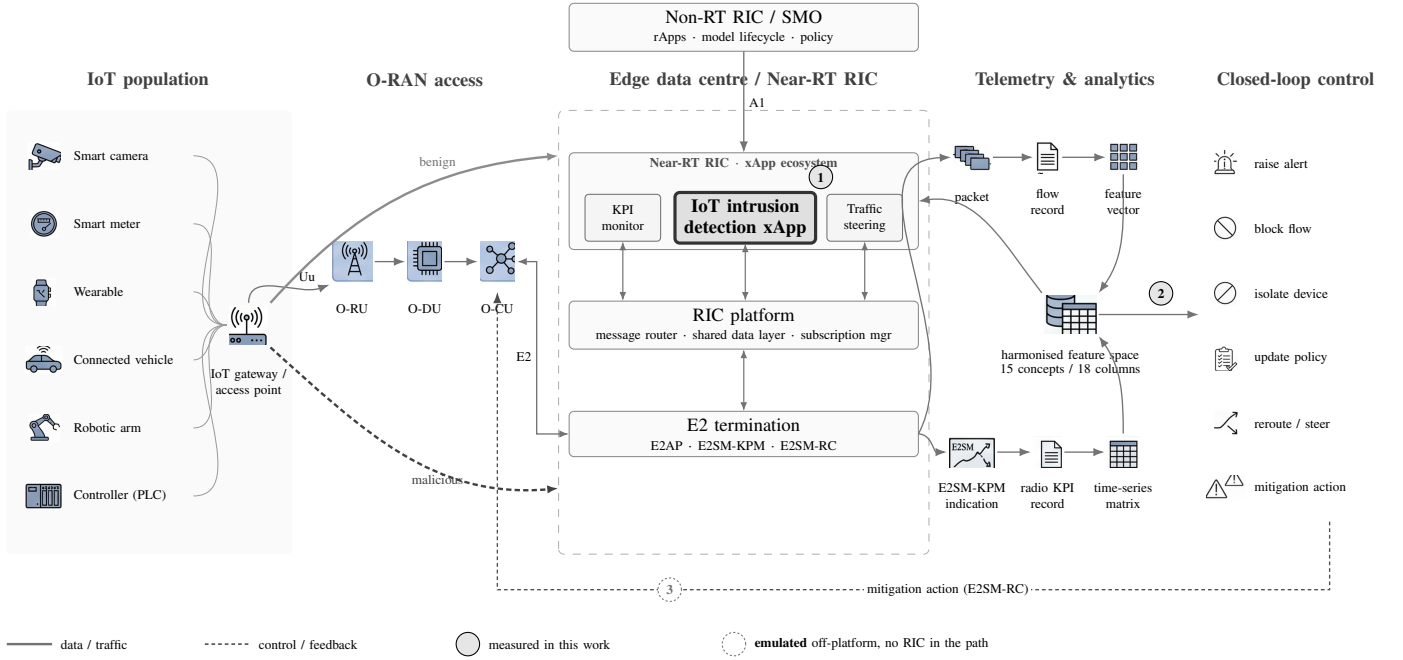
Fig. 1. Reference O-RAN edge deployment and the closed detection loop. The near-real-time RIC is hosted in a regional edge data centre and aggregates telemetry from many E2 nodes, so the detection xApp observes the combined behaviour of a large IoT population. Circled markers show where this paper takes its measurements: ① cross-deployment generalisation of the classifier and ② the alert burden imposed on the operator per unit time are measured; ③ decision latency against the near-real-time budget is emulated off-platform , with no RIC in the path, and supports relative ordering and stage decomposition only.
