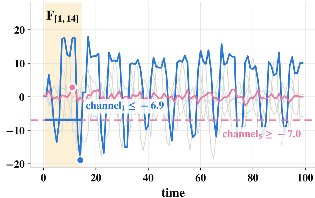
Predicted class: running (correct)
