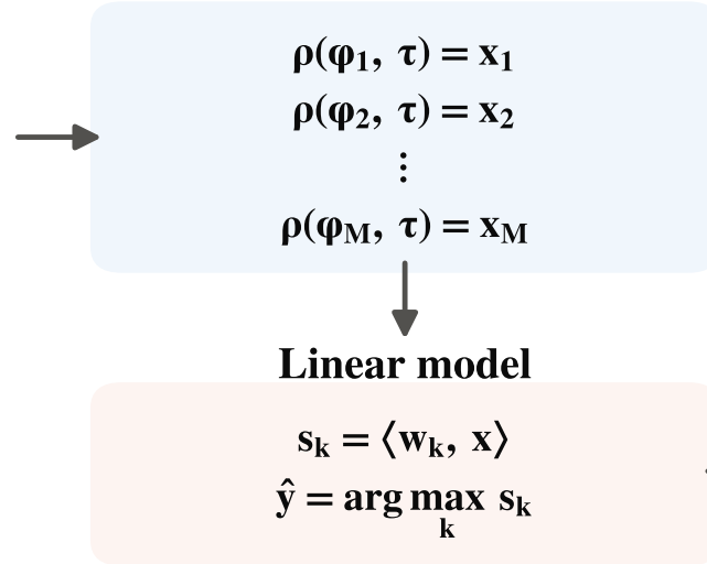
STL robustness features
