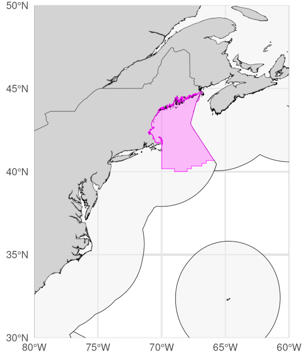
Figure 42: Shapefile for US Atlantic Halibut Stock
