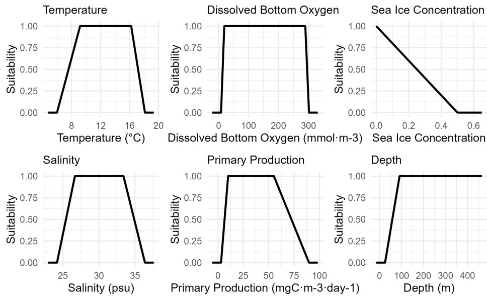
Figure 3: Environmental Envelopes for Greenstriped Rockfish
