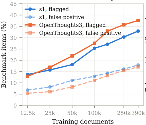
(a) Both rates rise with corpus size
