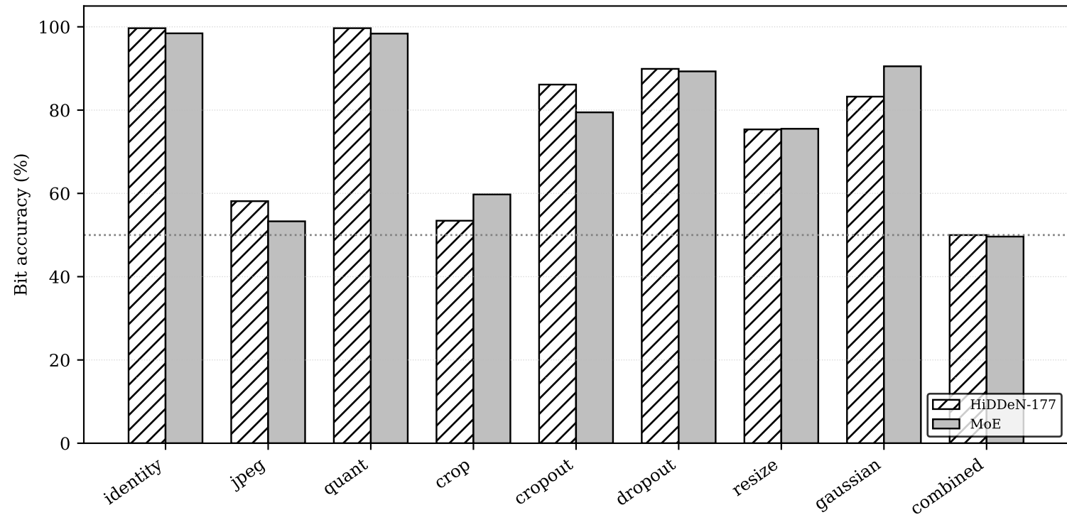
Attack robustness: 8exp k1 ep20
