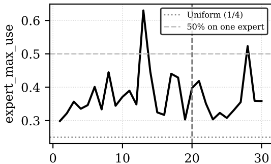
(e) Validation expert loads at epoch 20
