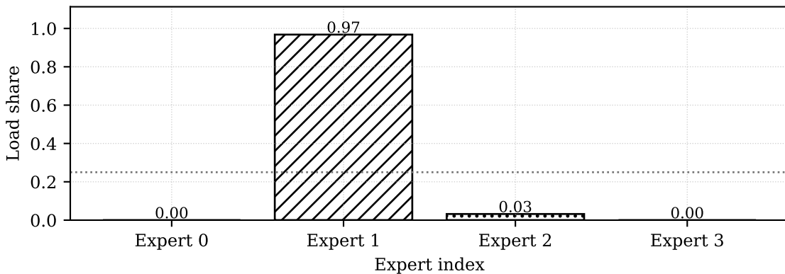
(e) Validation expert loads at epoch 13
