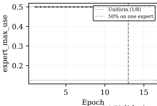
(e) Validation expert loads at epoch 13
