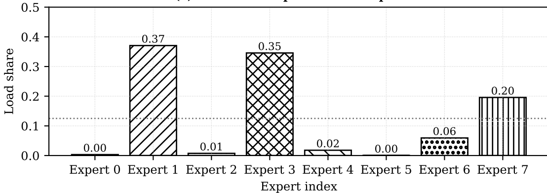
(e) Validation expert loads at epoch 3
