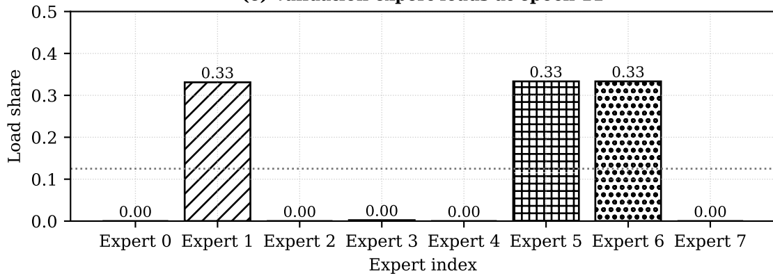
(e) Validation expert loads at epoch 11
