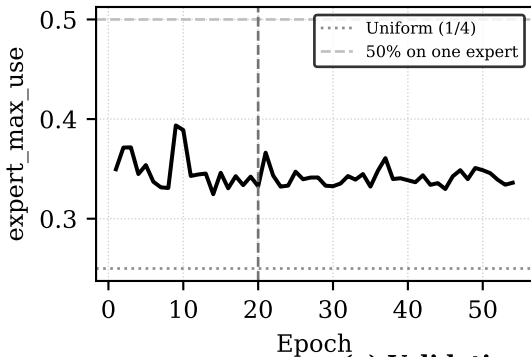
(e) Validation expert loads at epoch 20
