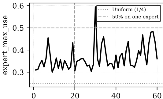
(c) Expert max use
