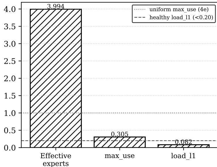
(b) MoE routing stability @ epoch 20
