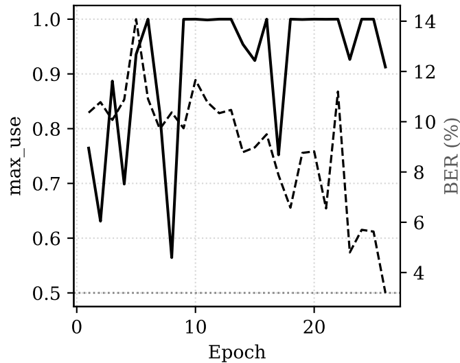
Mode 2: high jitter (balance v3)
