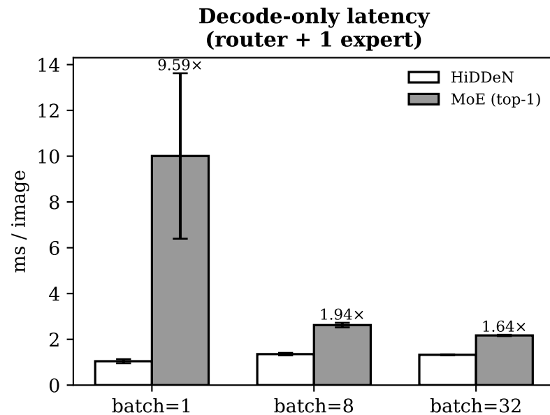
RQ4: MoE inference cost vs HiDDeN baseline (measured) Sparse top-k=1: only one expert decoded per image regardless of expert count.
