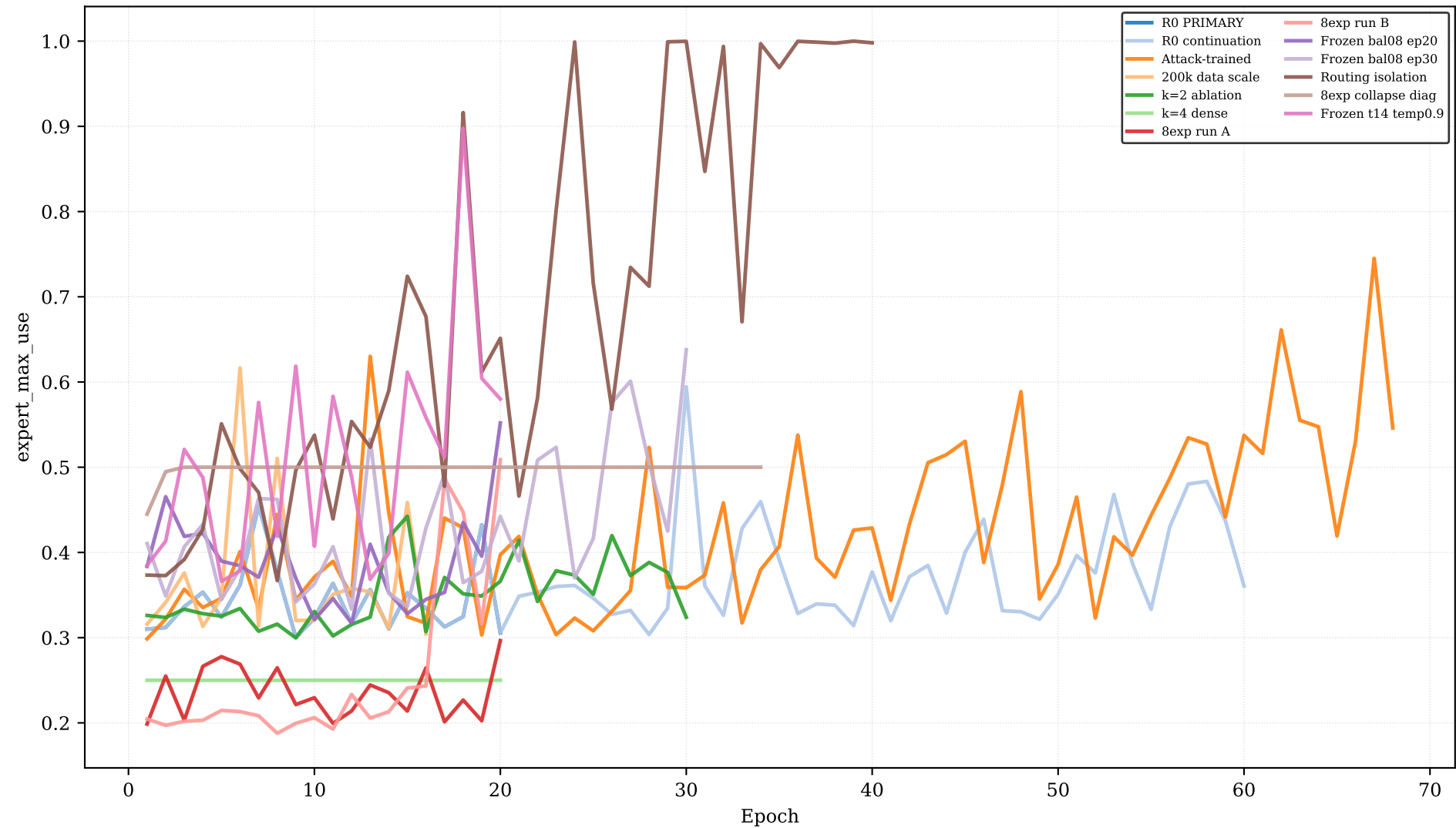
Expert max use — thesis runs (epoch 1 to final)
