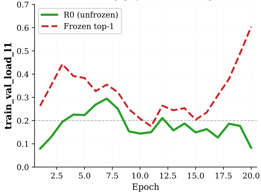
Routing gap over training
