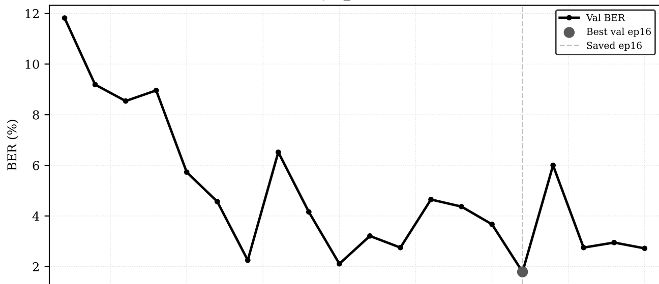
Frozen sym_bal08 (20 ep)
