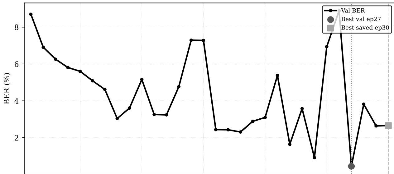
k=2 (top-2)
