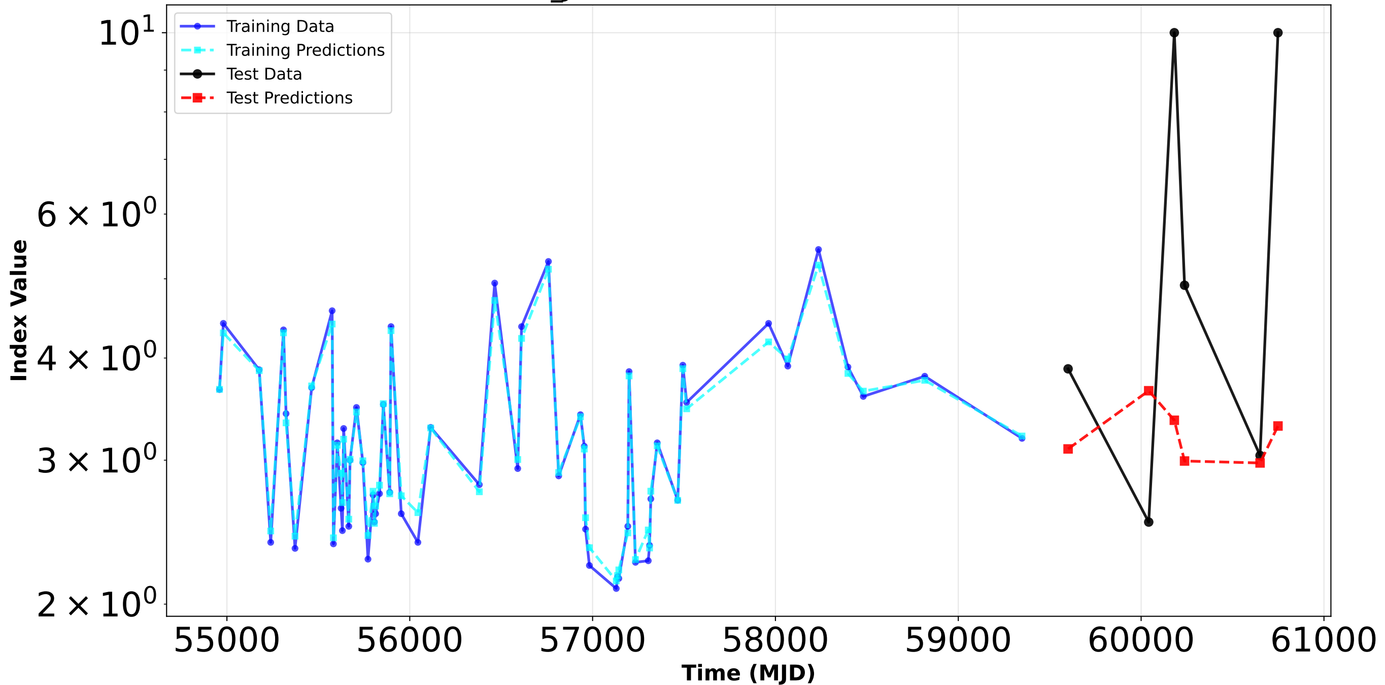
4FGL_J0009.3+5030 - INDEX Prediction
