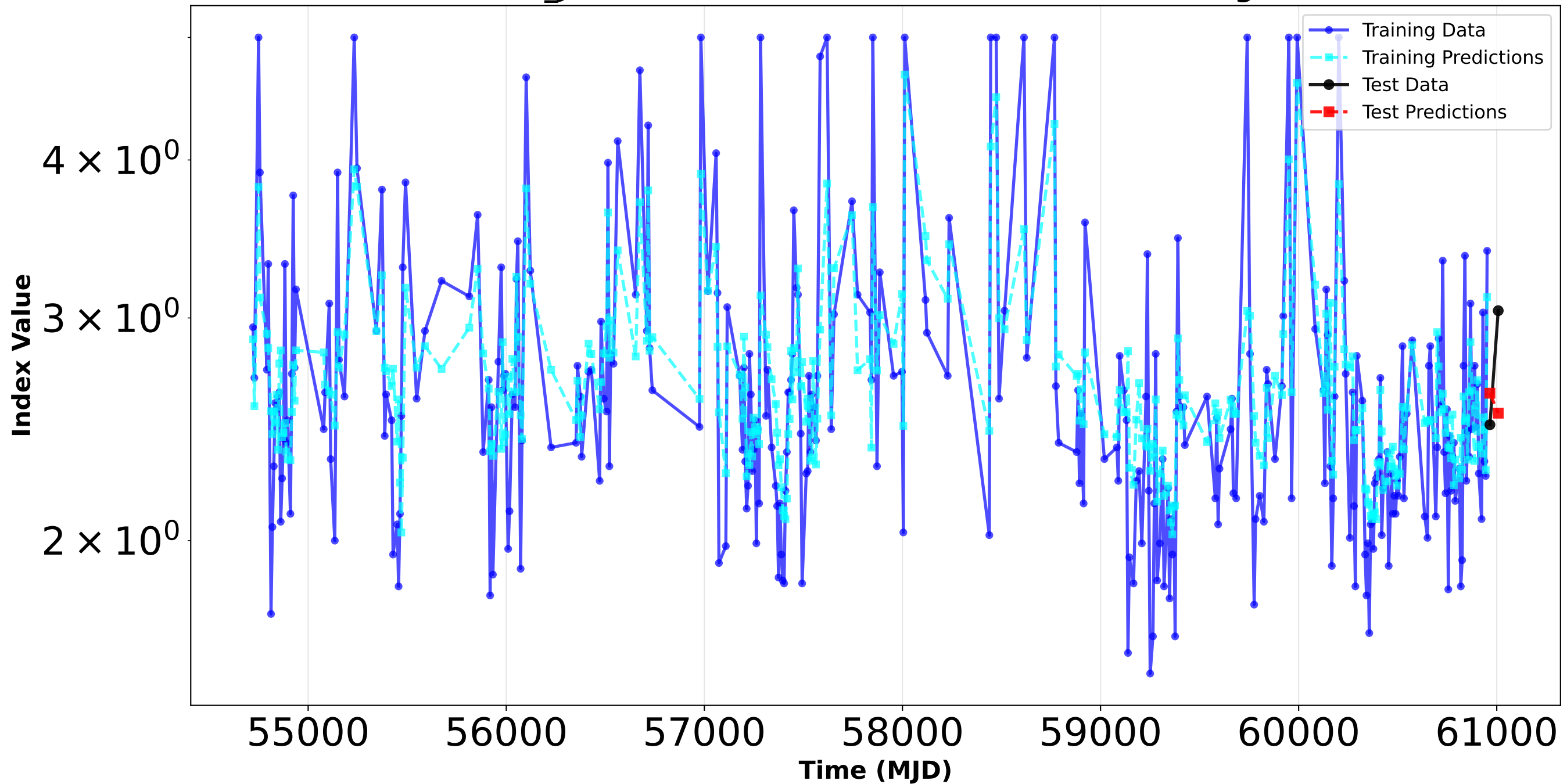
4FGL_J1321.1+2216 - INDEX Prediction (via Change)
