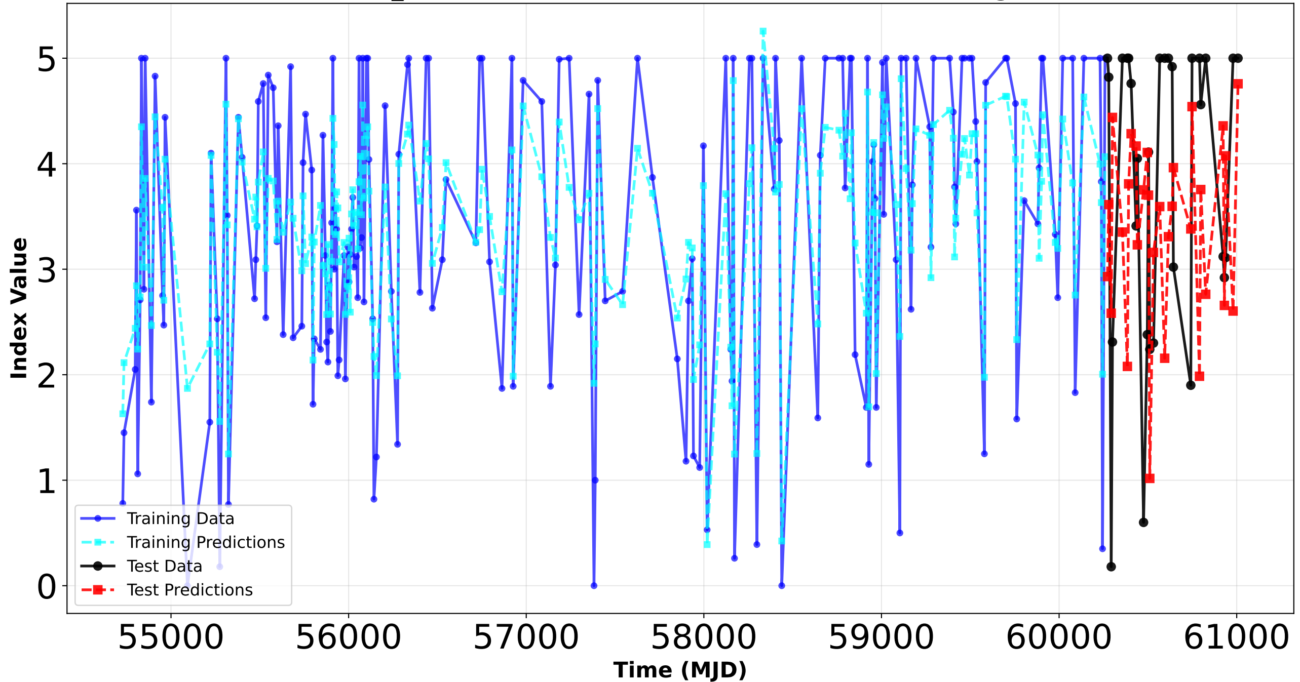
4FGL_J0001.5+2113 - INDEX Prediction (via Change)
