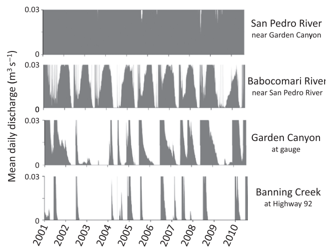
Fig. 2 Examples of differences in mean daily flow ( \text{m}^3 \text{s}^{-1} ) among stream types in the study region, as illustrated by 10 years of stream flow data (2001–10) from four different flow gauges in the region (see Fig. 1 for gauge locations). Peak discharges are truncated to maximise display of dry season differences. Stream reaches in our study area range from fully perennial (San Pedro River near Garden Canyon) to nearly perennial but with occasional dry periods (Babocomari River near San Pedro River), to intermittent with dry periods of several months (Garden Canyon at gauge), to intermittent with dry periods extending over many months and/or years (Banning Creek at Highway 92).
