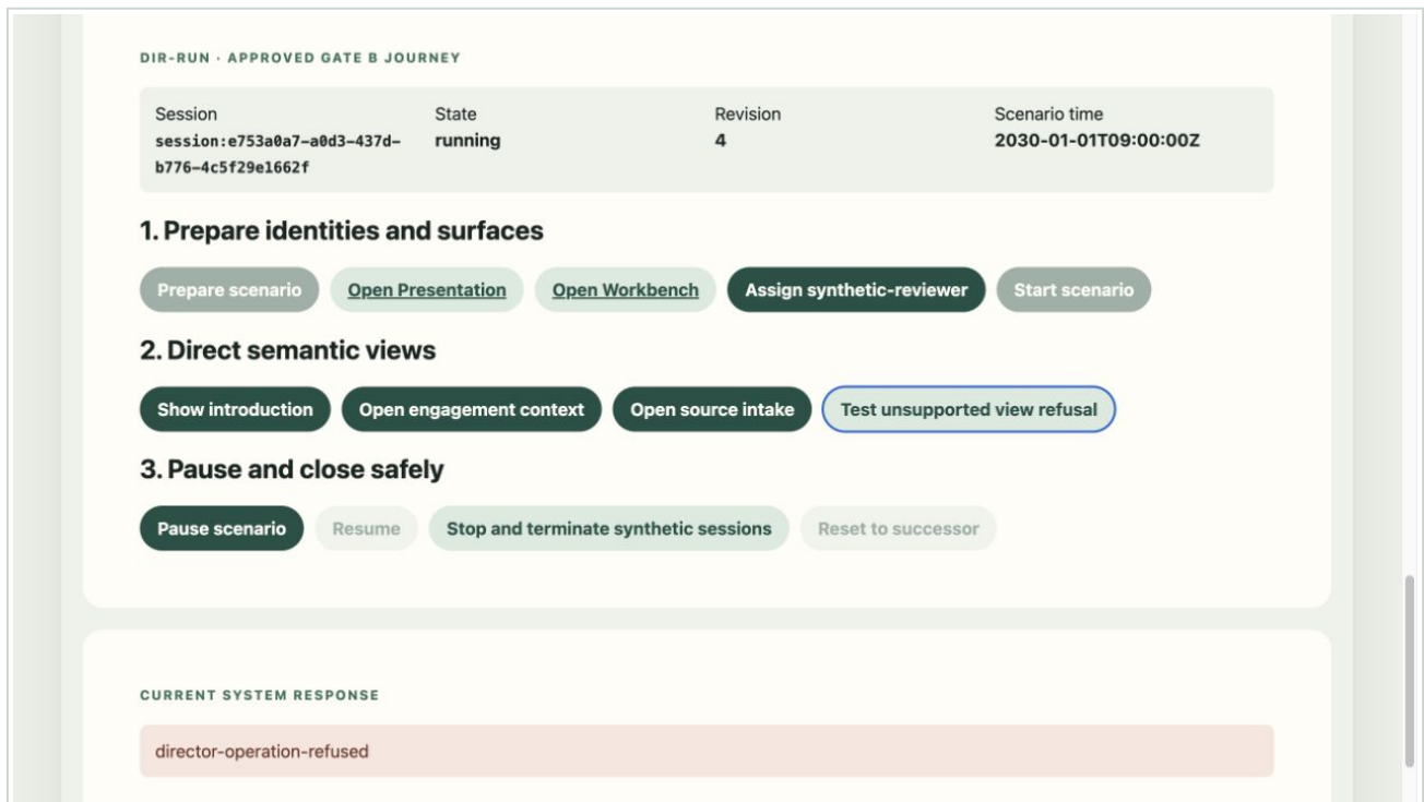
Figure 9. Explicit unsupported-view refusal in the Director.
