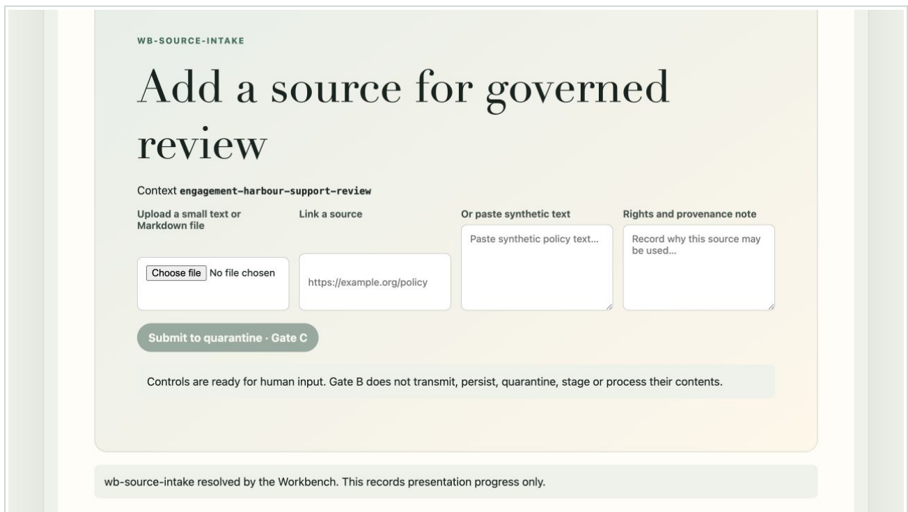
Figure 8. Director-requested source-intake view with Gate C submission disabled.
