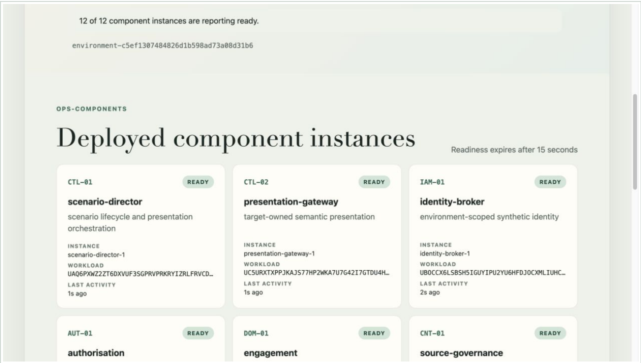
Figure 14. Operations component-mesh readiness view.
