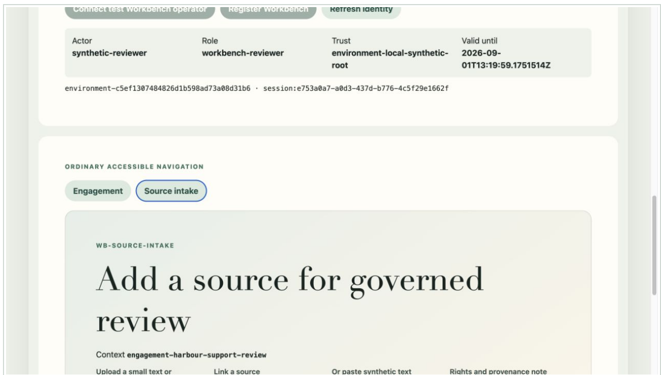
Figure 7. Manual navigation to source intake, explicitly recording that no business event was emitted.
