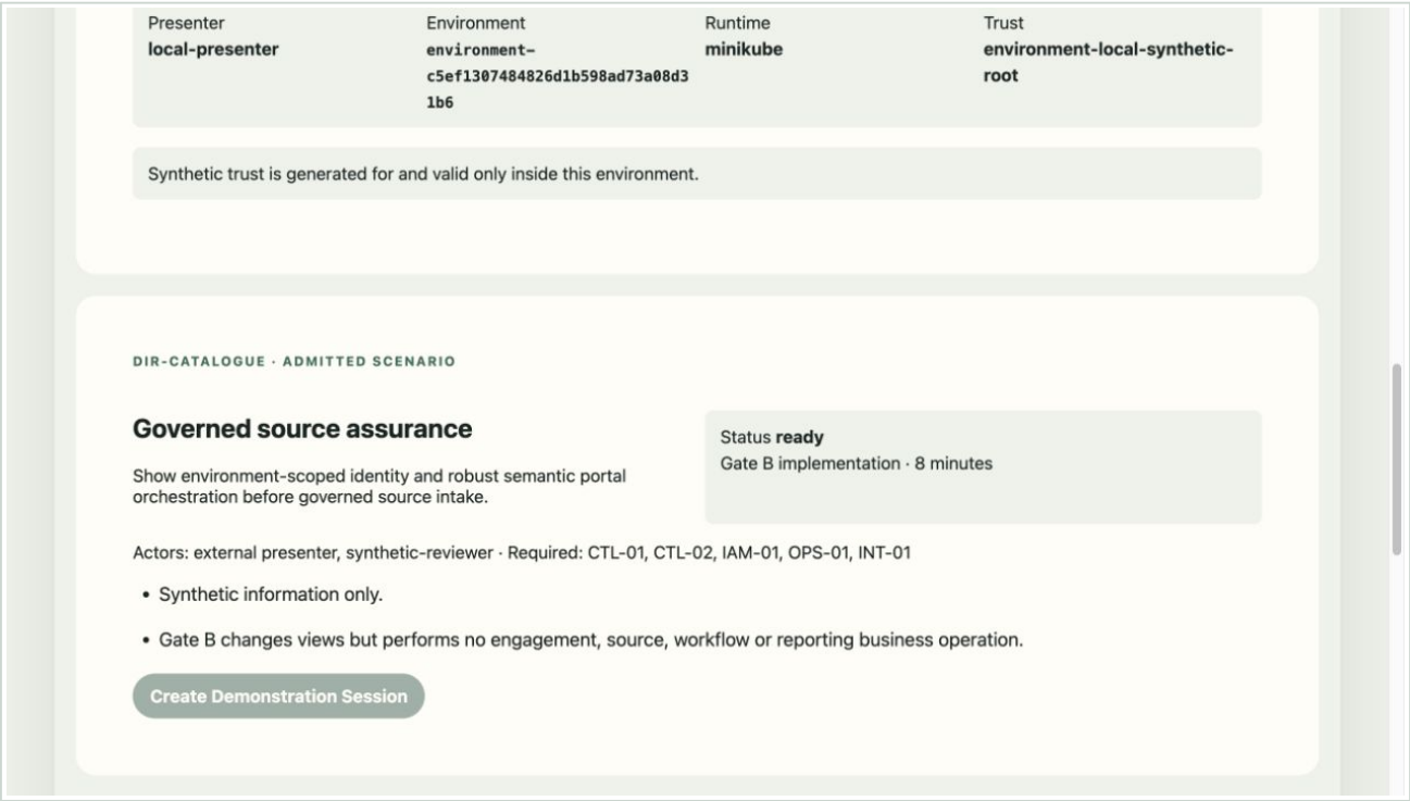
Figure 1. Director environment, environment-local synthetic trust and admitted governed-source scenario.
