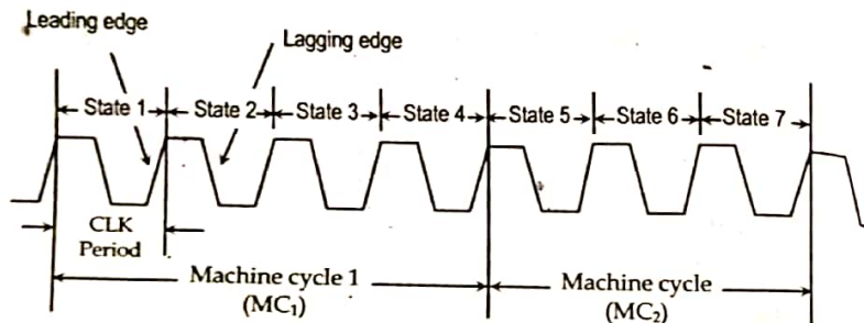
Figure: Machine cycle showing clock periods.
