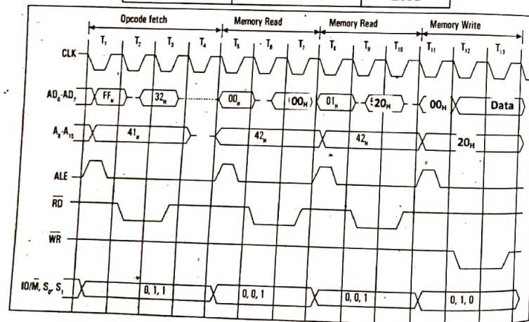
Figure: Timing diagram of instruction STA 2000H.
