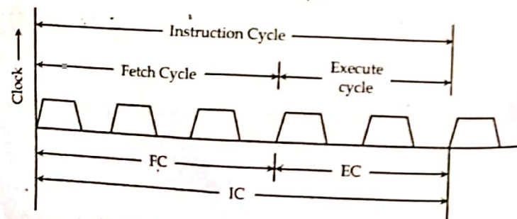
Figure: (b) Instruction cycle showing FC, EC and IC
