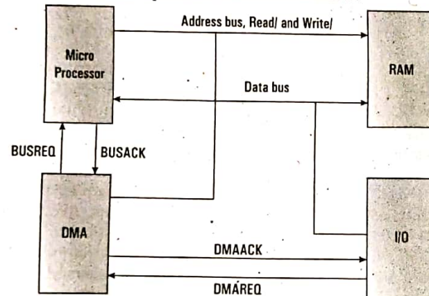
Figure: Illustration for DMA transfer in a computer system
