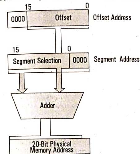
Figure: Real addressing mode
