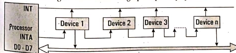
Figure: Chained interrupt handling.
