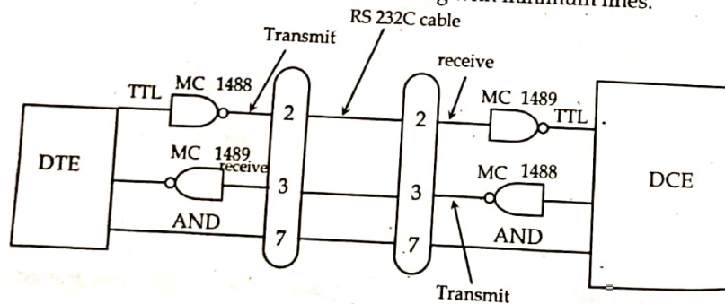
Figure: RS 232C interface
