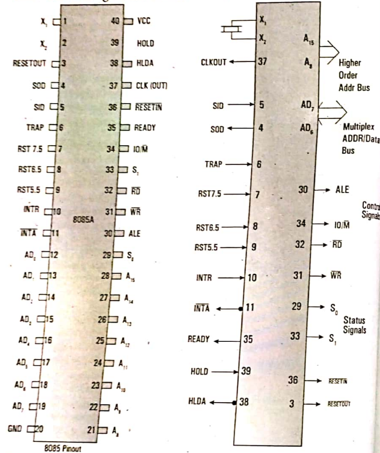
Figure: PIN Configuration of 8085
