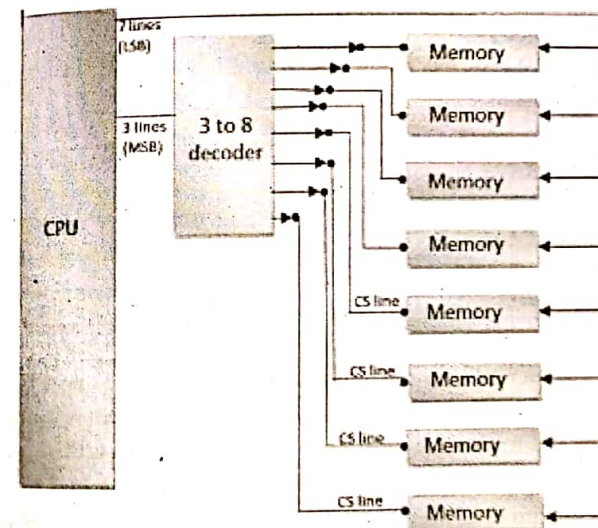
Figure: 3 to 8 address decoding.
