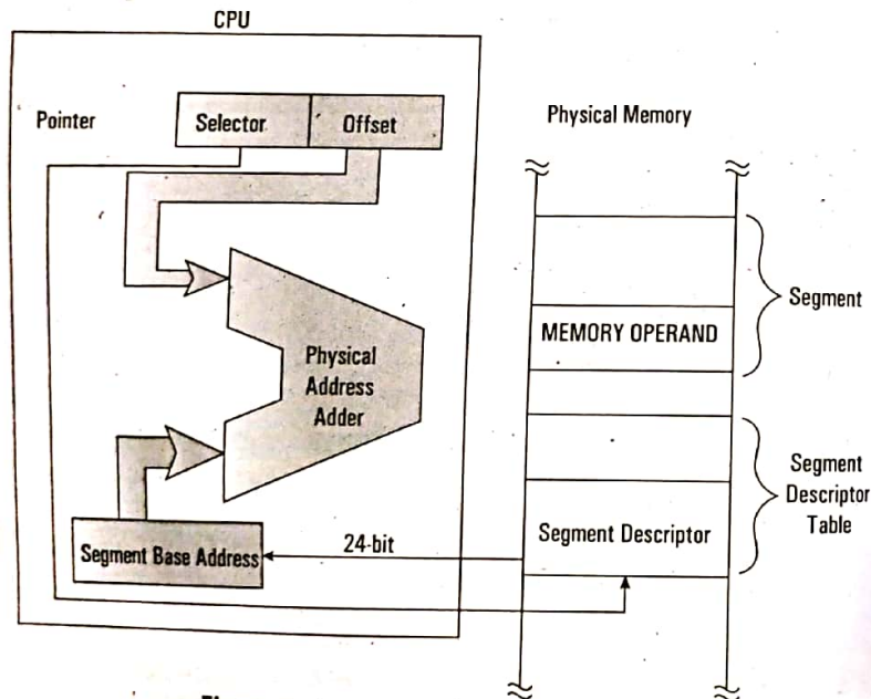
Figure: Protected virtual addressing mode
