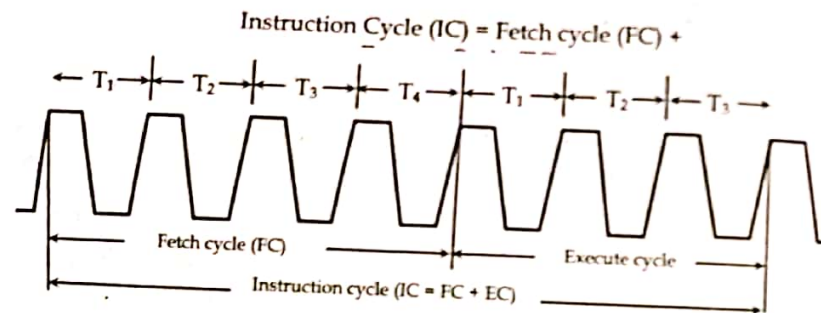
Figure: (a) Processor cycle
