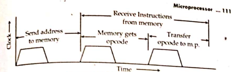
Figure: (c) A Typical Fetch cycle
