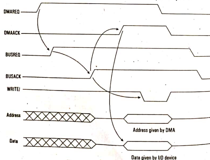
Figure: DMA Timing Diagram
