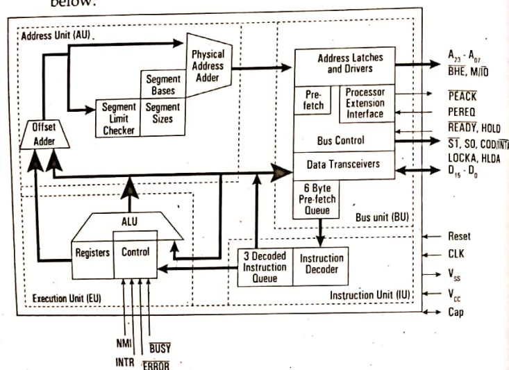
Figure: Internal Block Diagram of 80286
