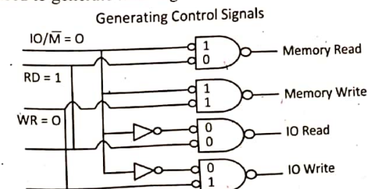
Figure: Generating Control Signals
