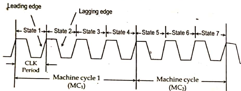
Figure: Machine cycle showing clock periods.
