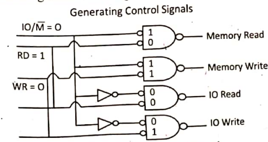
Figure: Generating Control Signals
