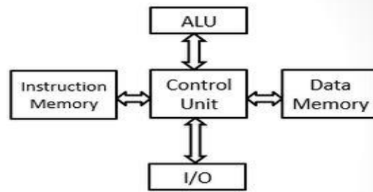
Harvard Model
