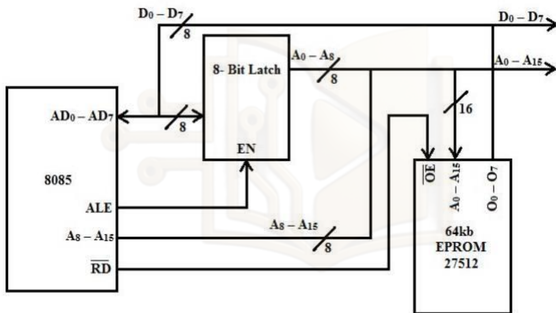
Fig 1.6 Memory Interfacing
