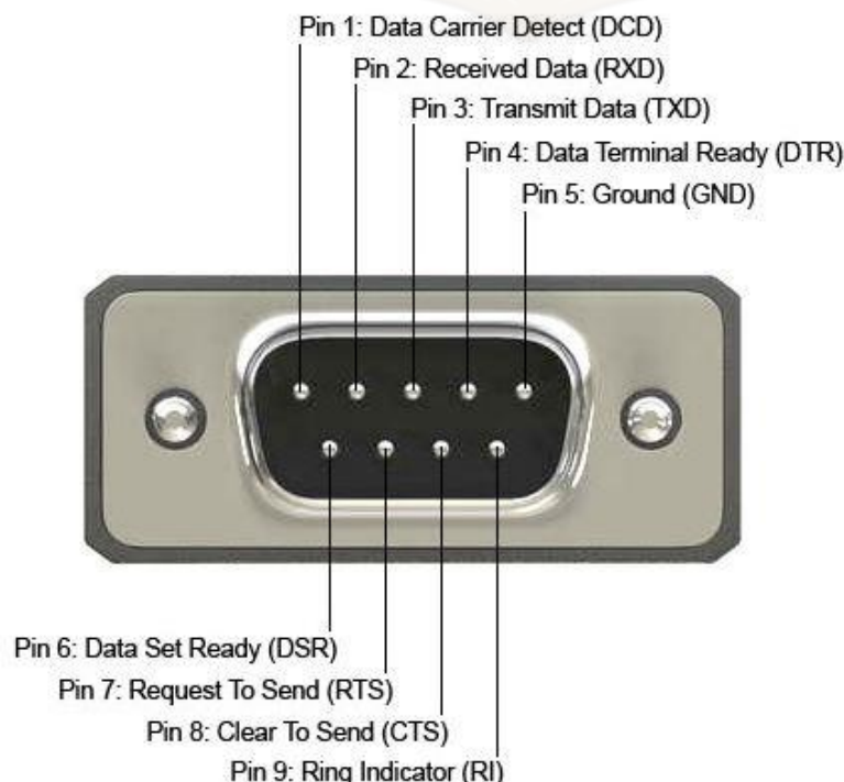
RS232 Pinout
