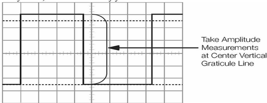
Figure: Measure voltage on the center vertical graticule line.
