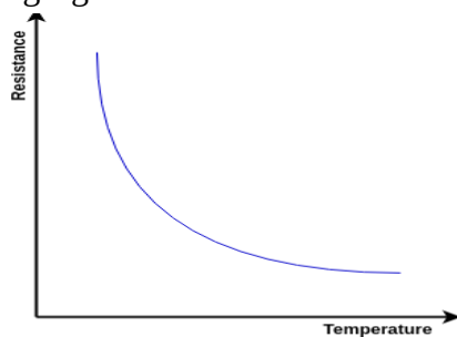
NTC Characteristics
