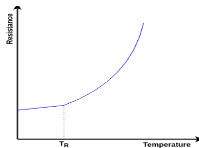
PTC Characteristics
