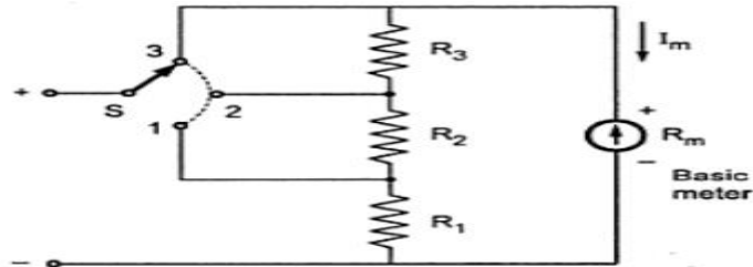
Fig. 1 Ammeter with Ayrton shunt
