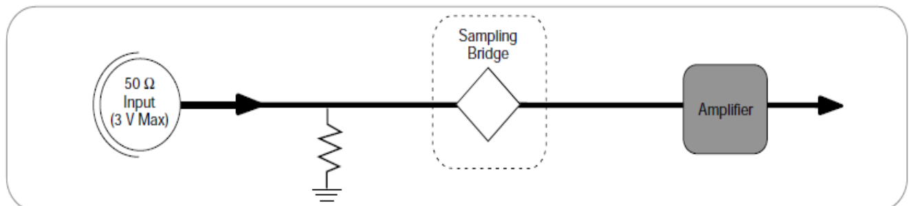
Fig: The Architecture of a Digital Sampling Oscilloscope.
