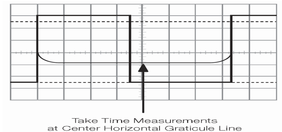
Figure: Measure Time on the Center Horizontal Graticule Line.
