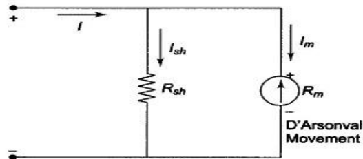
Fig: Basic DC Ammeter
