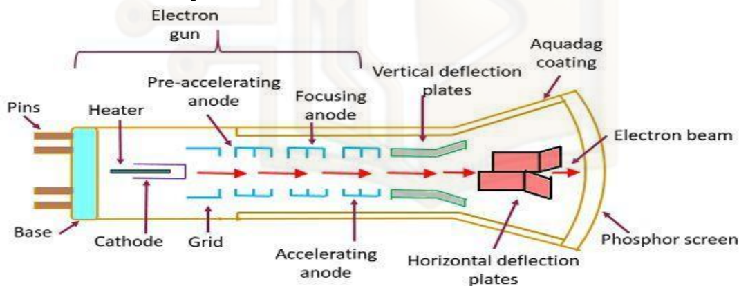
Fig: Internal Structure of CRT
