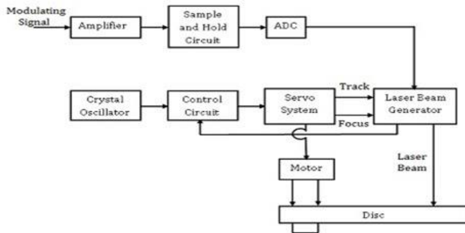
Figure: Block Diagram of CD Recording
