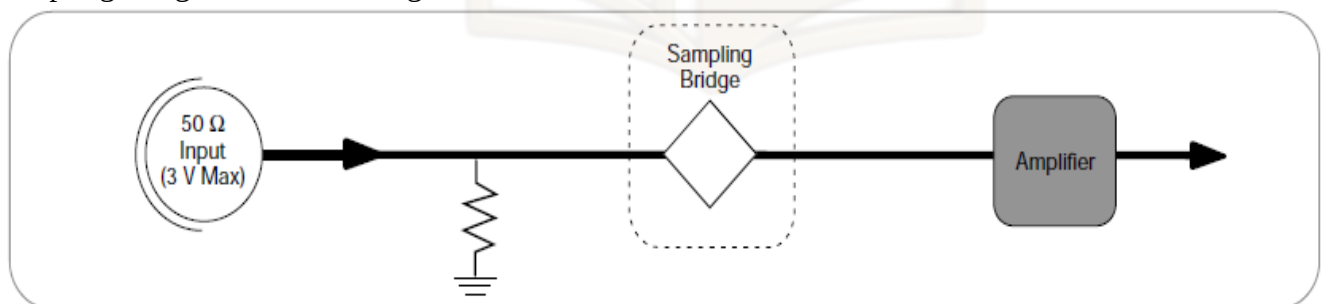
Fig: The Architecture of a Digital Sampling Oscilloscope.
