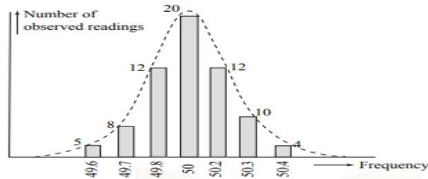
Figure: Histogram showing distribution of parameter readings
