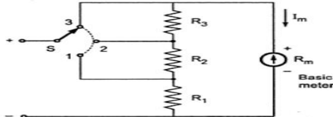
Fig. 1 Ammeter with Ayrton shunt
