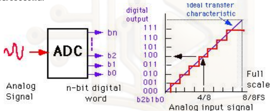
Fig: Analog to Digital Conversion Process
