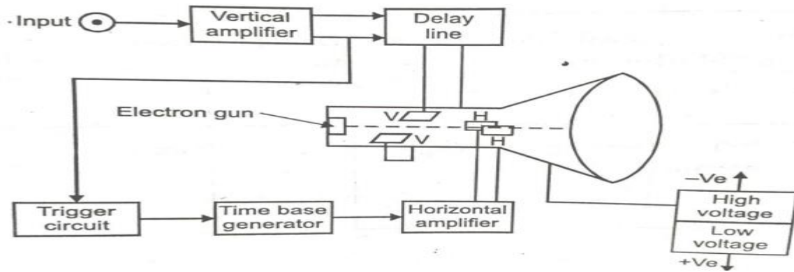
Fig: Block Diagram of oscilloscope
