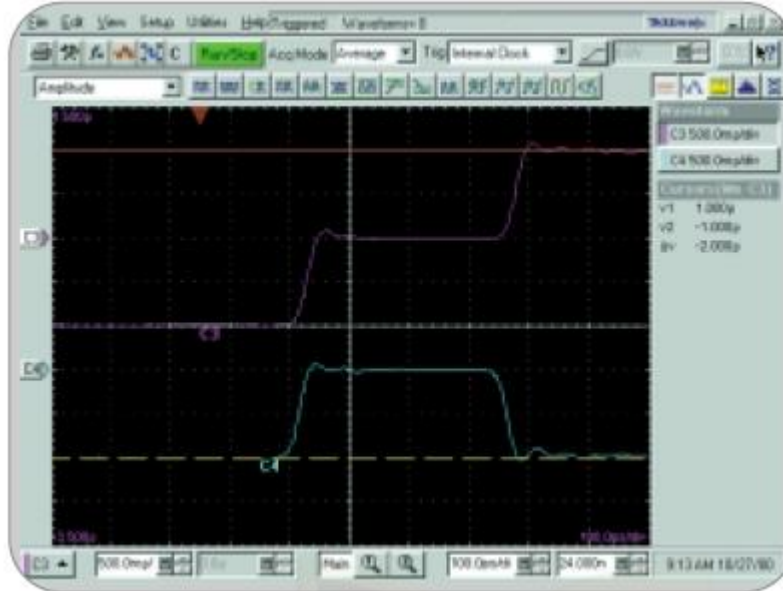
Time domain reflectometry (TDR) display from a TDS8000 digital sampling oscilloscope and 80E04 20-GHz sampling module.
