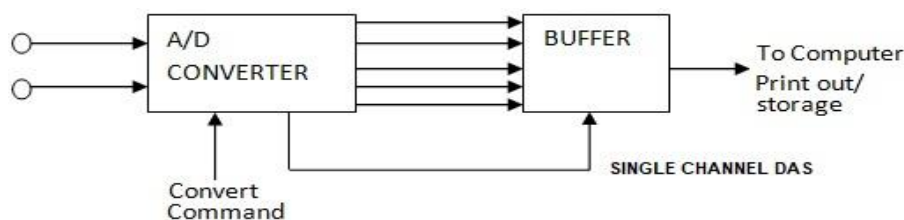
Fig: Block Diagram of Single Channel DAS
