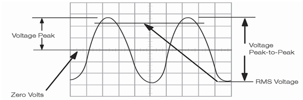
Figure: Voltage Peak ( V_p ) and Peak-to-Peak Voltage ( V_{p-p} ).
