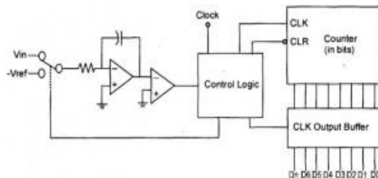
Fig: Dual Slope Analog to Digital Converter
