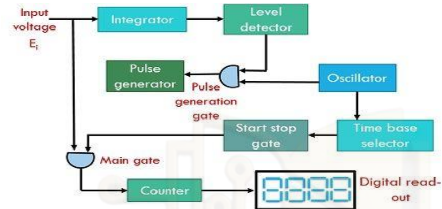
Block diagram of integrating type DVM
