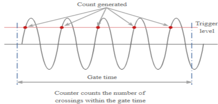
Basic concept of a frequency counter
