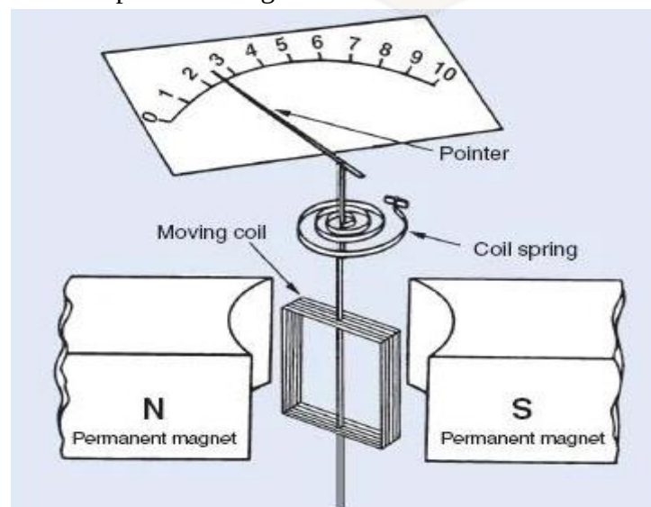
Figure: Exploded view of a moving-coil movement
