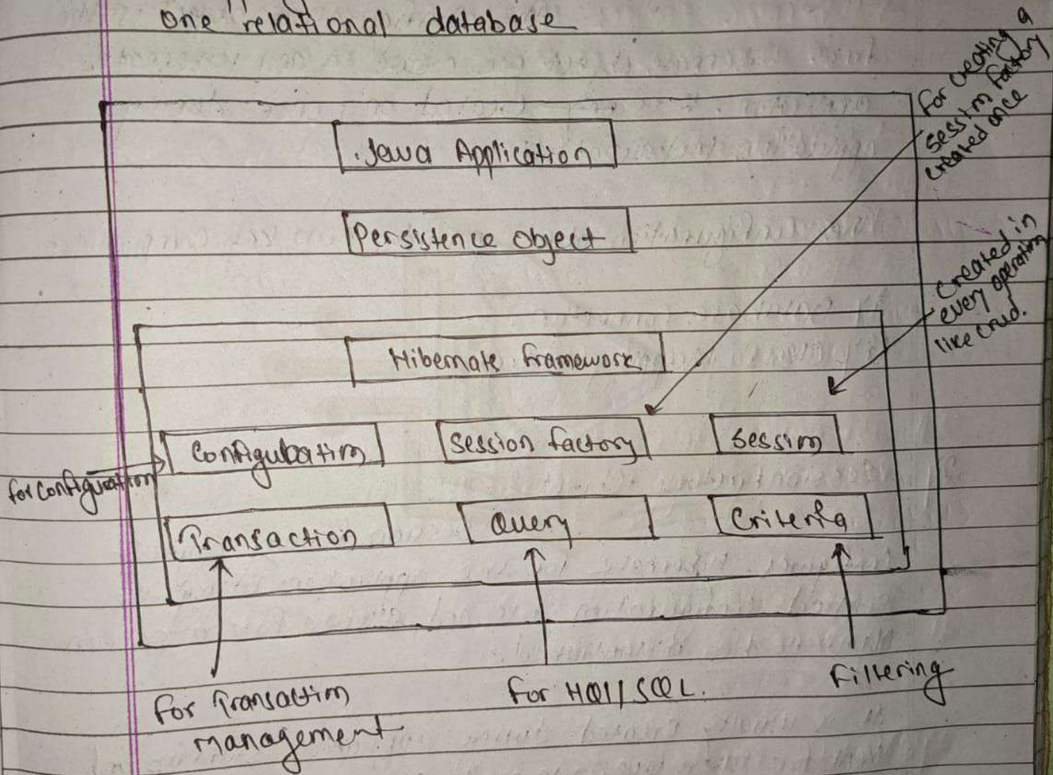
Fig 8- Hibernate Architecture
