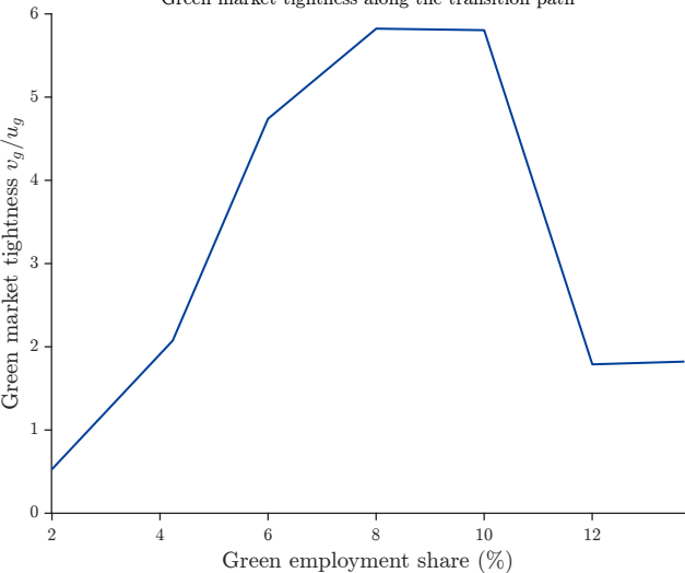
Green market tightness along the transition path
