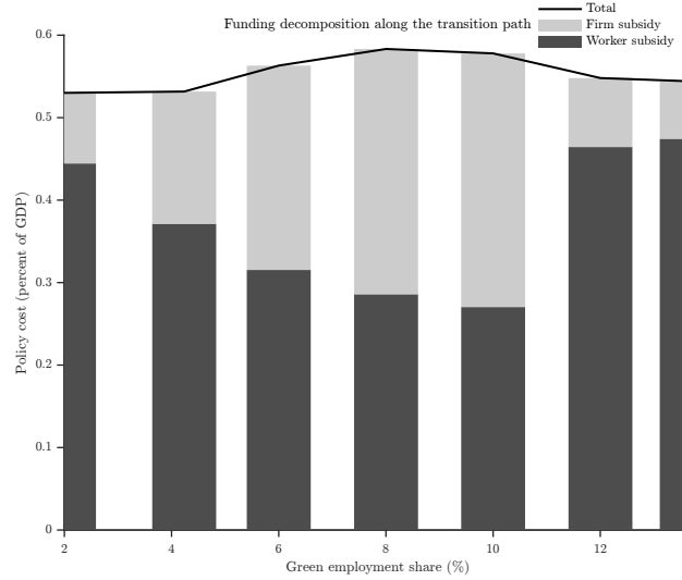
Figure 7. Funding decomposition along the same path: worker support vs. firm subsidies; line shows total funding as a percent of GDP.
