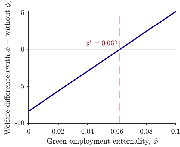
Figure 6. Welfare effects as a function of the externality parameter \phi (threshold \phi^* \approx 0.062 ).
