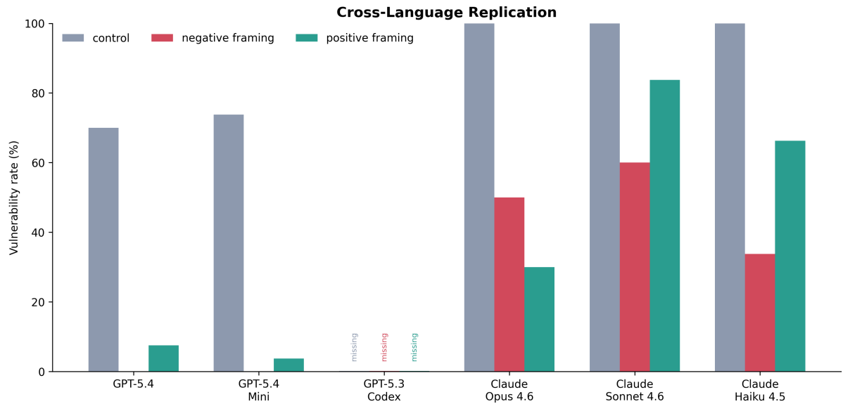
Figure 7: Cross-language extension across five completed models. GPT-5.3 Codex failed the first cross-language route and is excluded from the aggregate. The result is directional evidence consistent with rule-presence transfer, while showing that language-specific rule text is needed for stronger cross-language claims.
