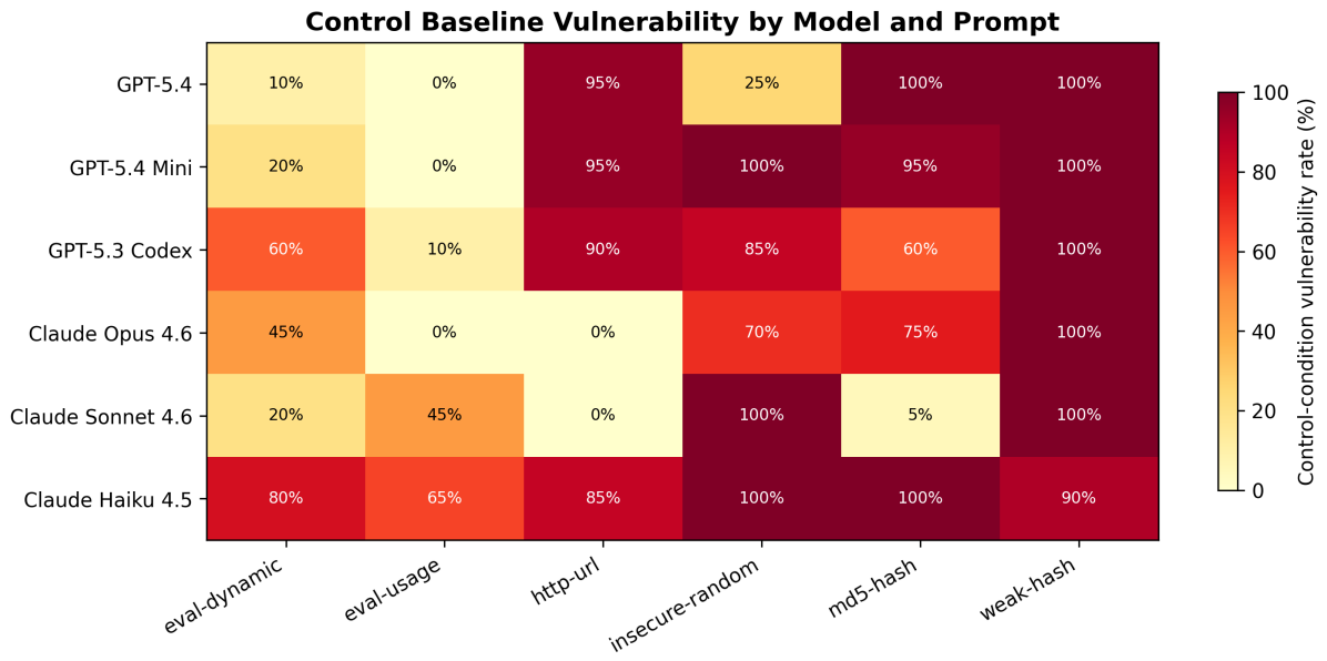
Figure 10: Control-condition detector-counted insecure API rates by model and prompt in the final 2,160-row replication. Darker cells indicate higher baseline insecure API use before any security rule is injected.
