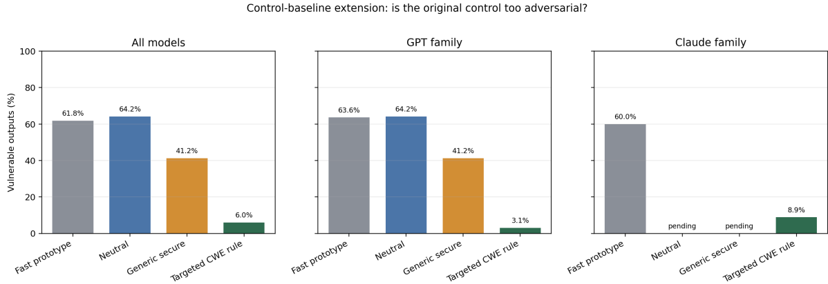
Figure 6: Bounded control-baseline sensitivity. In the completed GPT-5.4 plus GPT-5.4 Mini slice, the neutral helper control closely matches the original fast-prototype control, generic security advice helps partially, and the targeted combined rule remains much lower. Claude-family neutral/generic controls are still incomplete, so this figure is a bounded sensitivity check rather than a full replacement main result.
