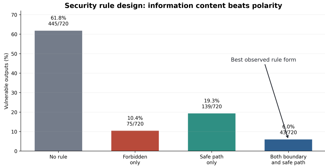
Figure 8: Practical rule-design takeaway from the four-arm extension. The safest observed rule form states both the unsafe boundary and the safe replacement path.
