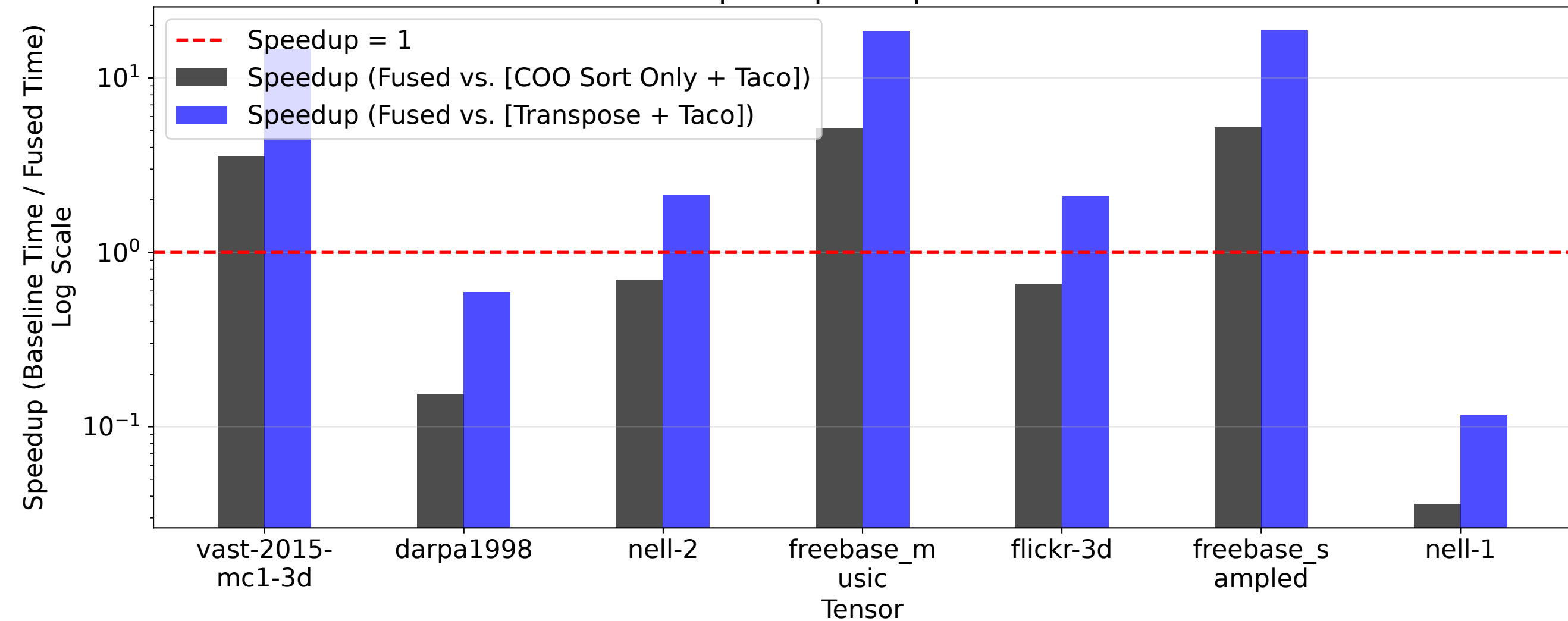
Speedup Comparison
