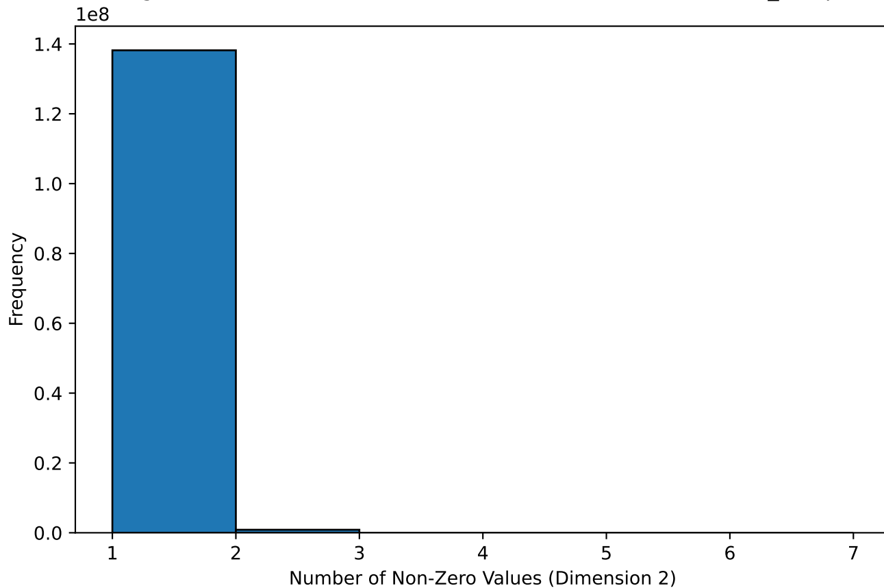
Histogram of Non-Zero Counts in Second Dimension (freebase_sampled)
