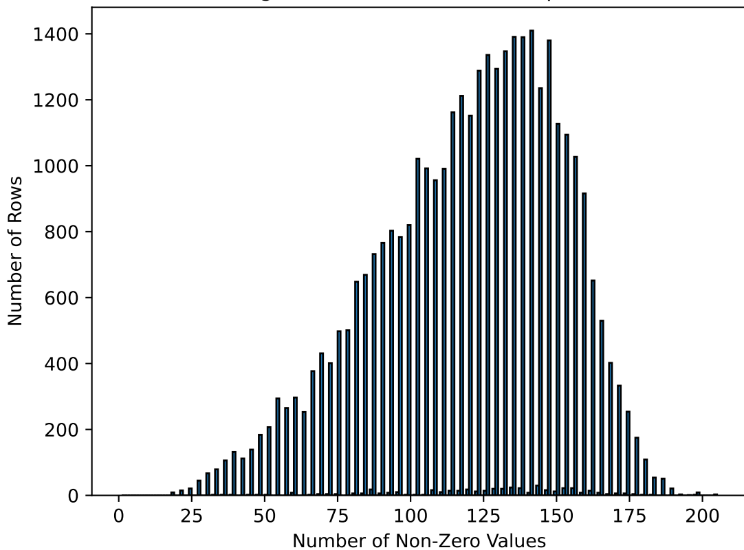
Histogram of Non-Zero Counts per Row
