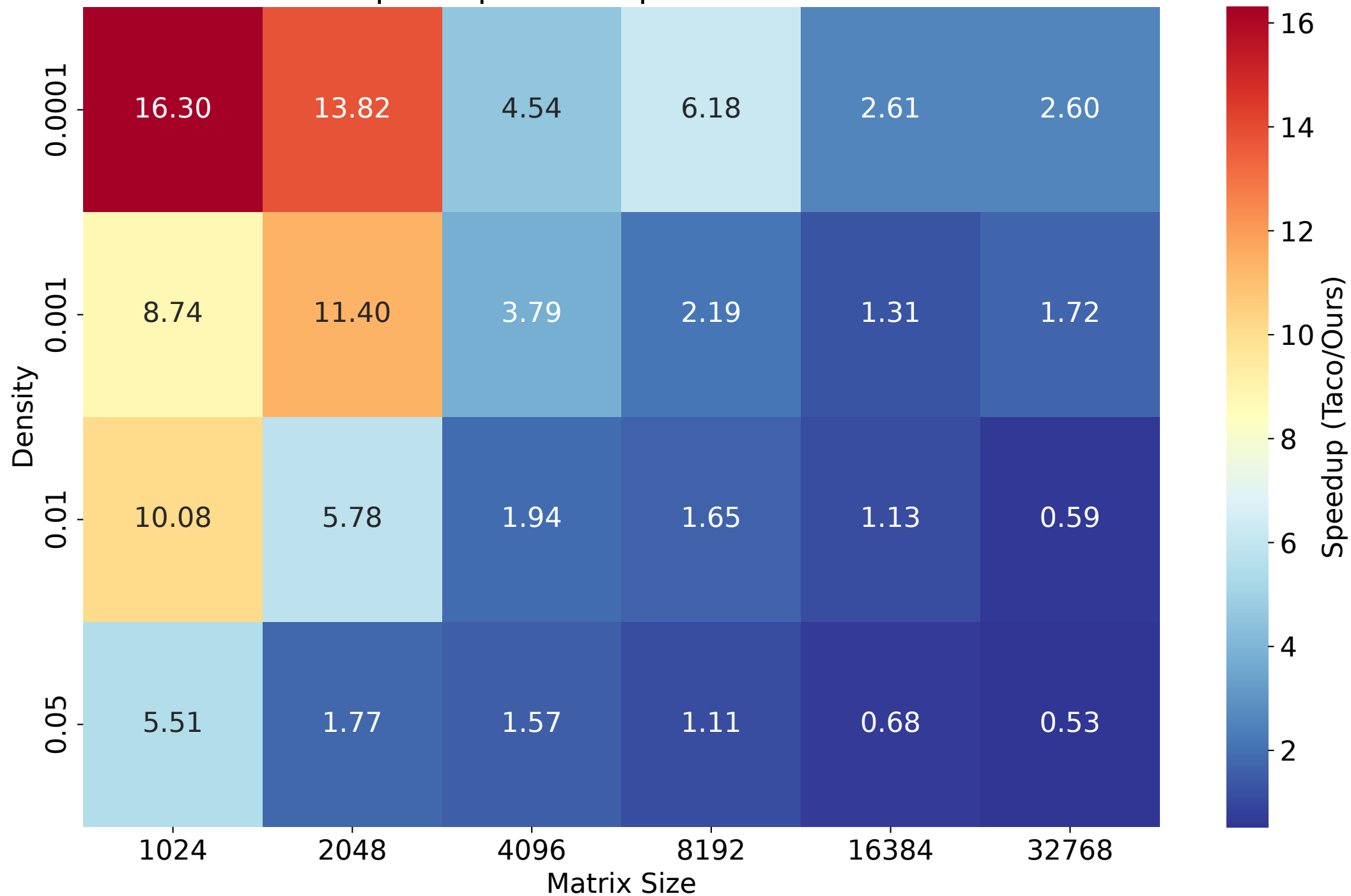
Speedup Heatmap: Taco vs Ours
