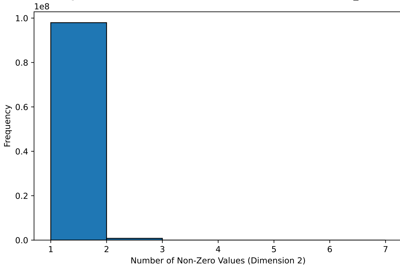
Histogram of Non-Zero Counts in Second Dimension (freebase_music)
