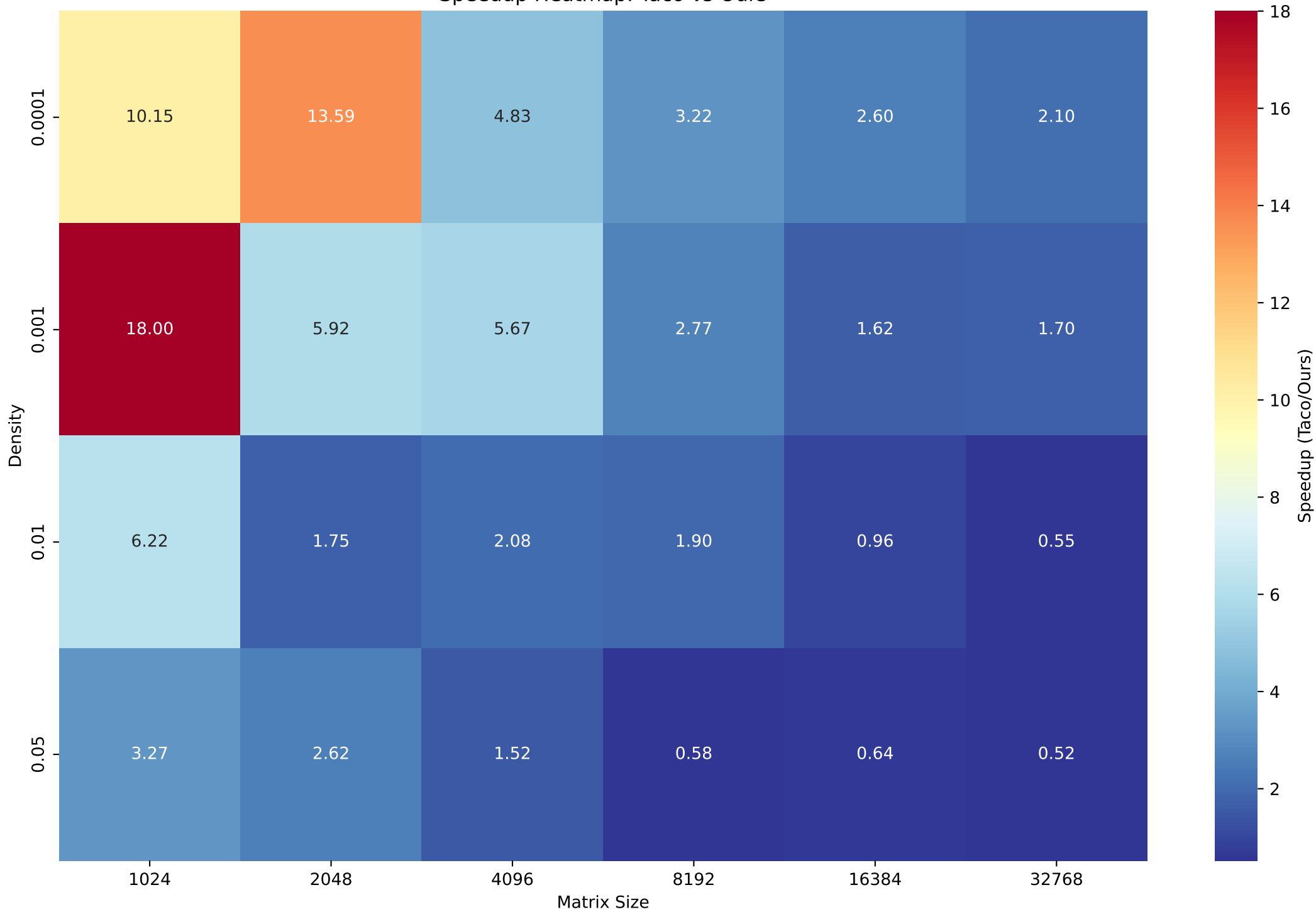
Speedup Heatmap: Taco vs Ours
