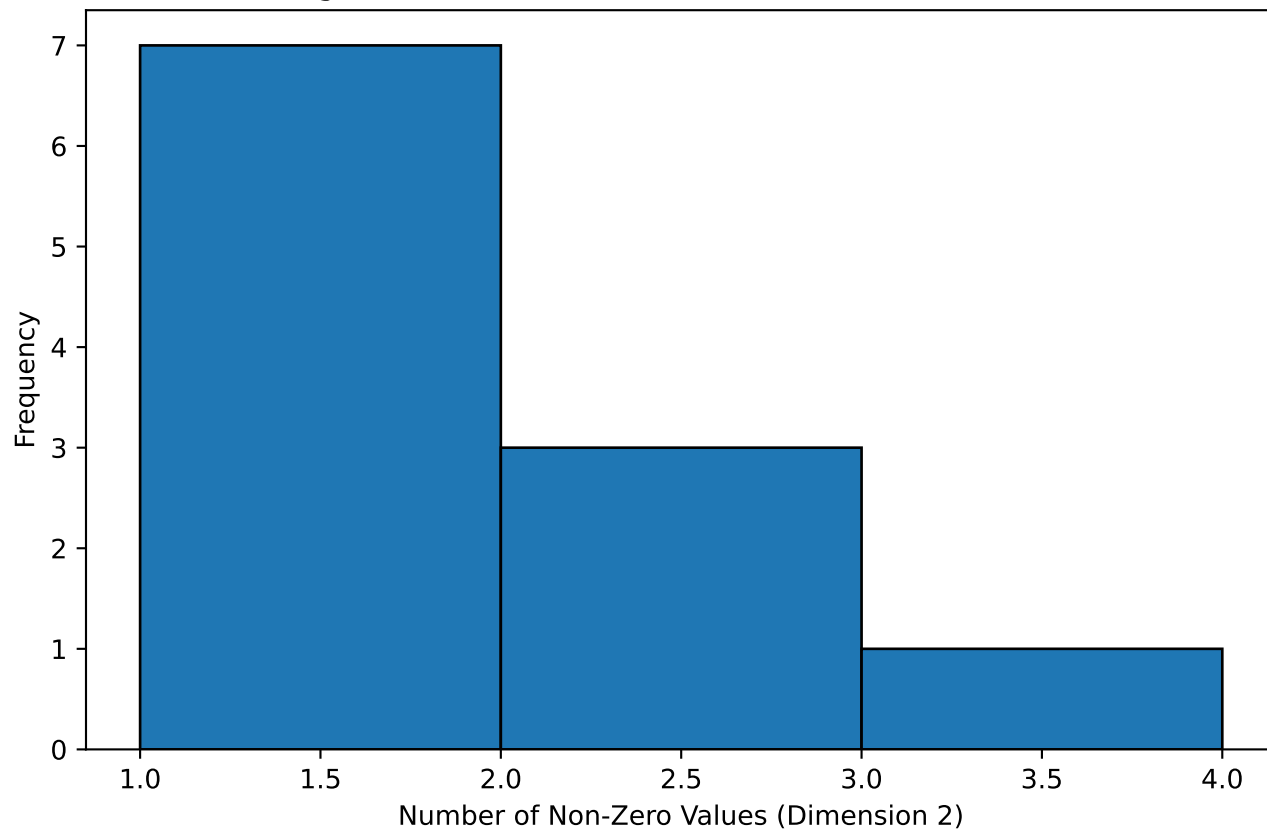
Histogram of Non-Zero Counts in Second Dimension (A)
