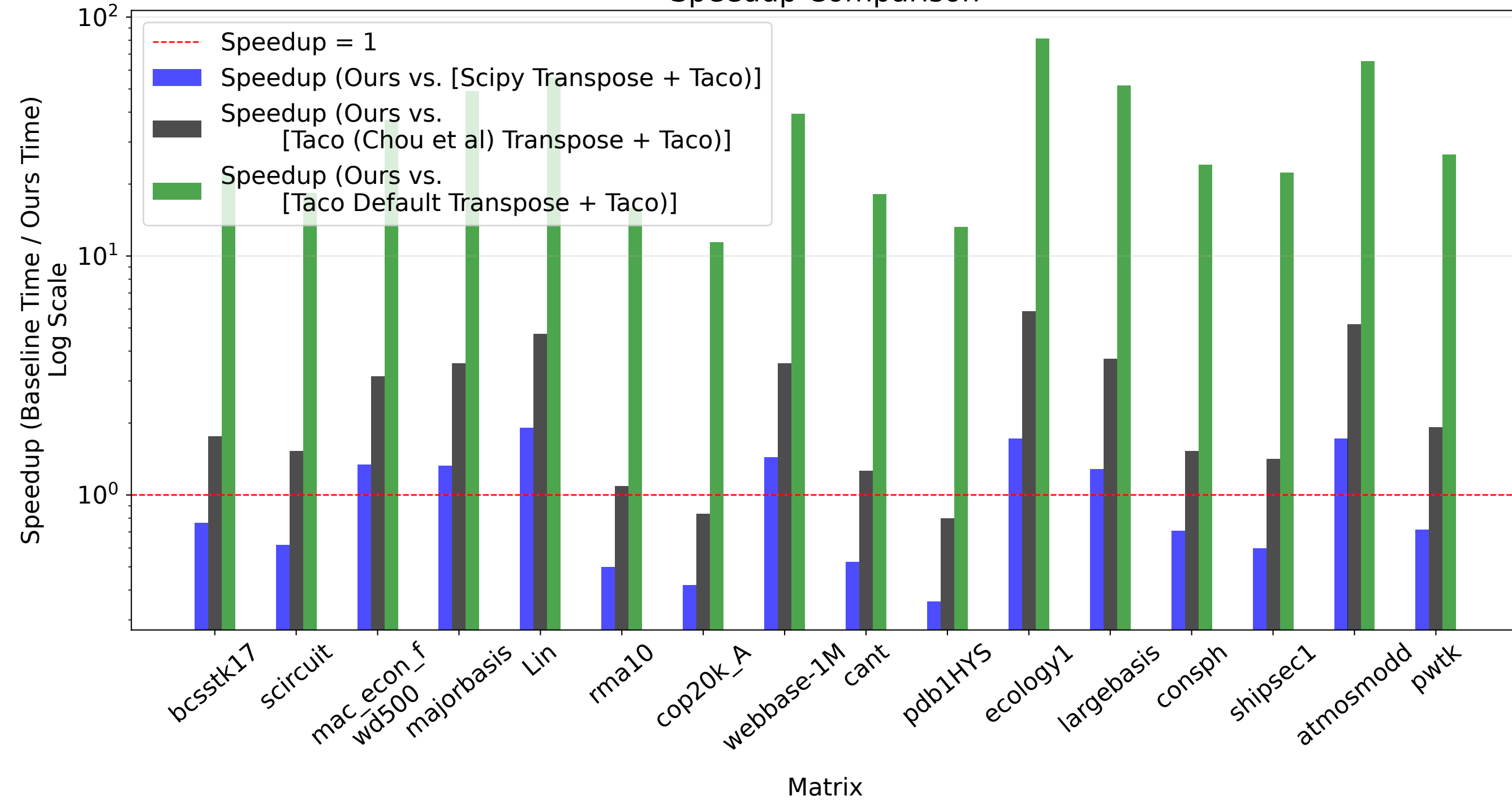
Speedup Comparison
