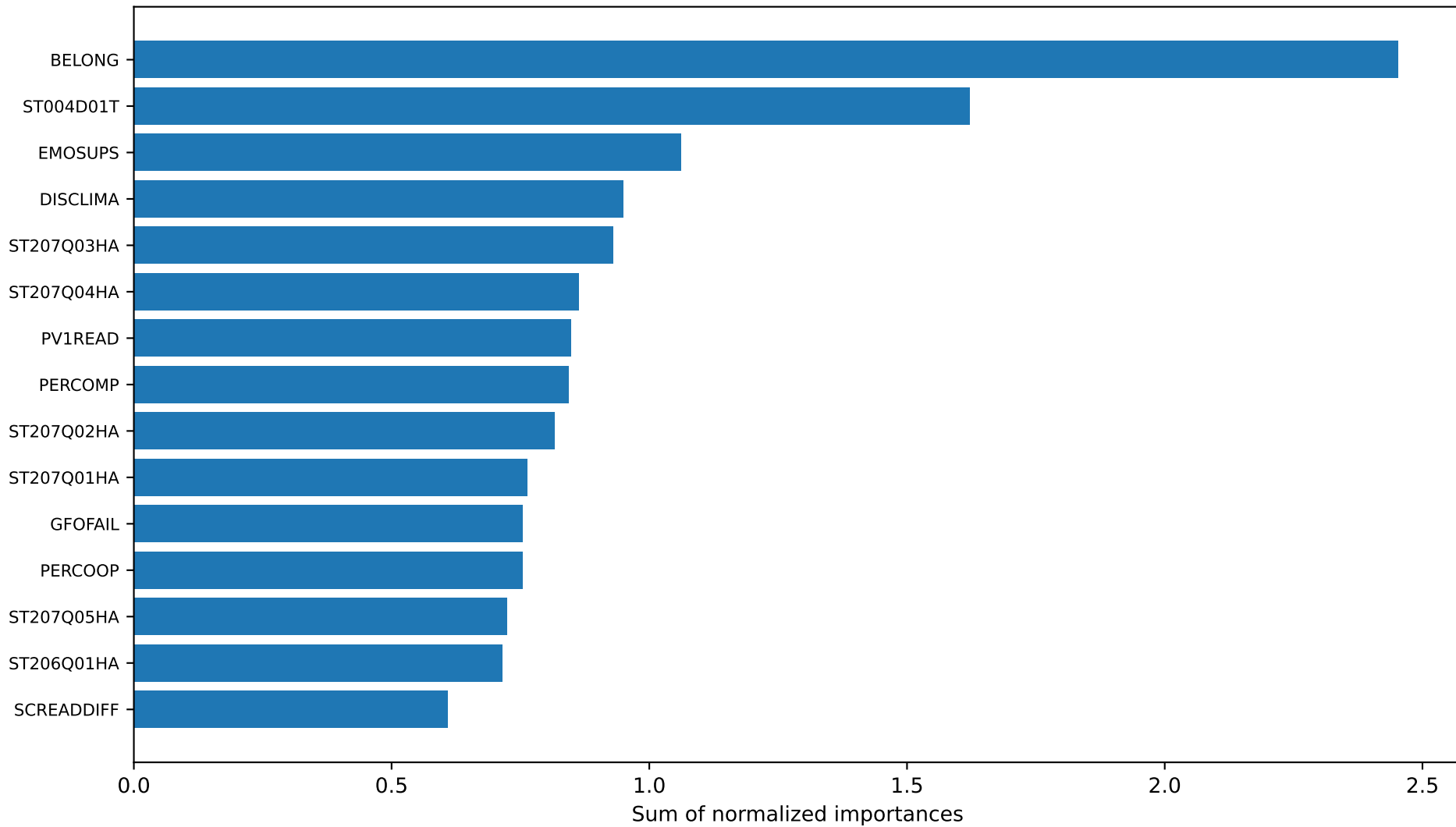
Aggregate Predictors by Cluster — BEINGBULLIED (Full ranking, normalized) — Cluster 1
