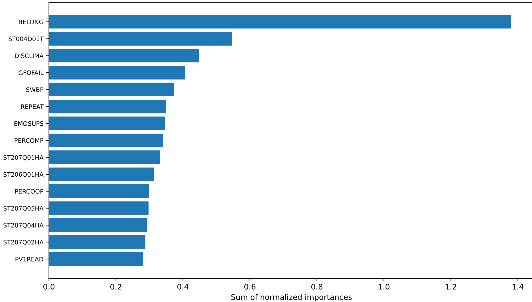
Aggregate Predictors by Cluster — BEINGBULLIED (Full ranking, normalized) — Cluster 0
