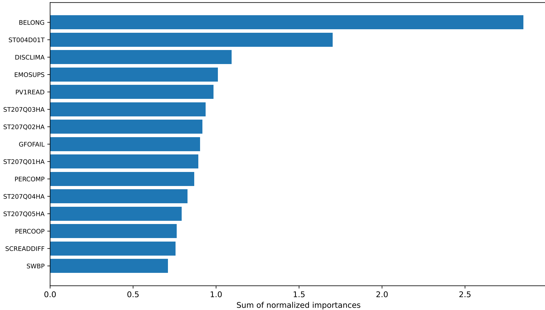
Aggregate Predictors by Cluster — BEINGBULLIED (Full ranking, normalized) — Cluster 2
