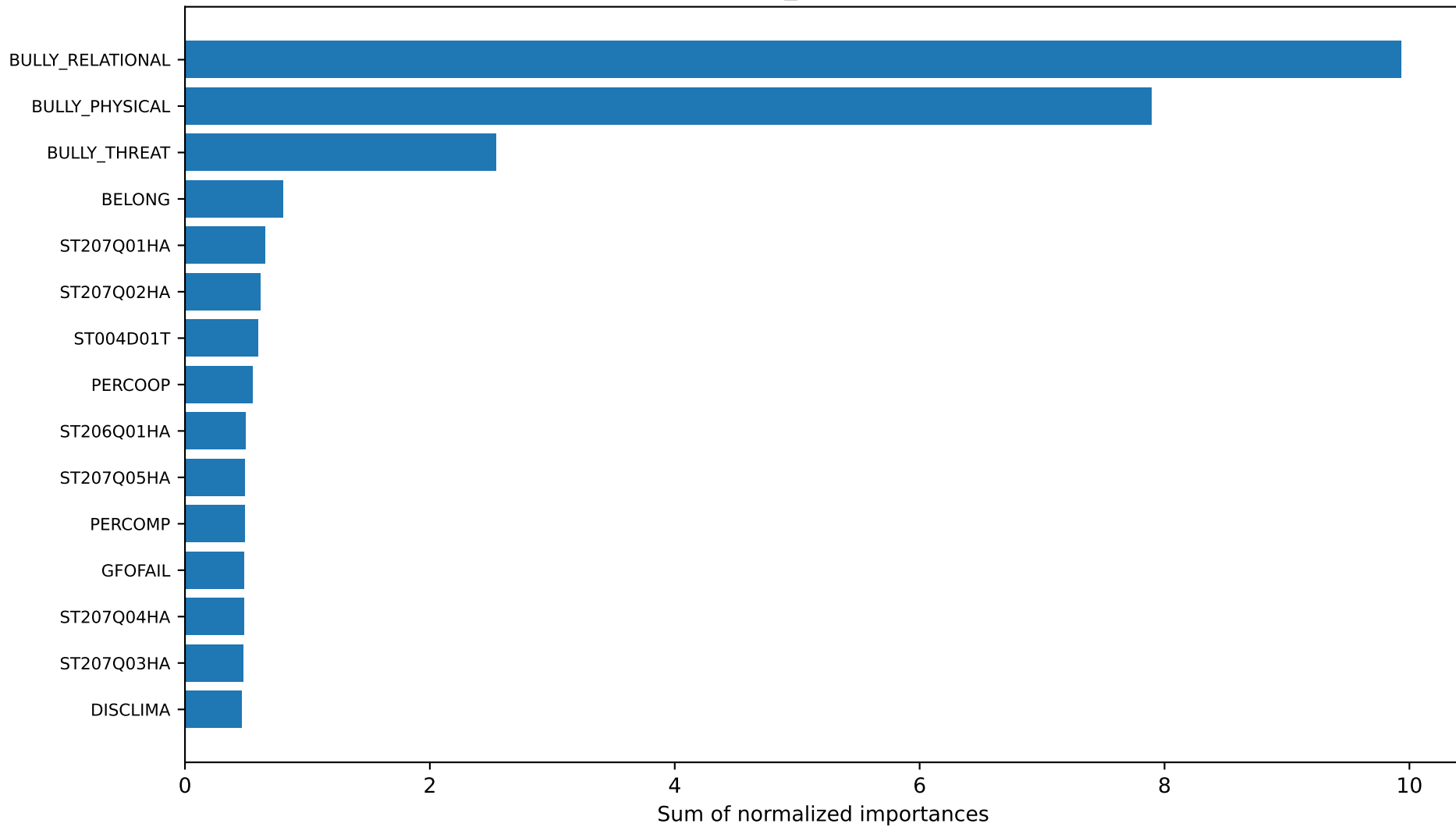
Aggregate Predictors by Cluster — BULLY_VERBAL (Full ranking, normalized) — Cluster 0
