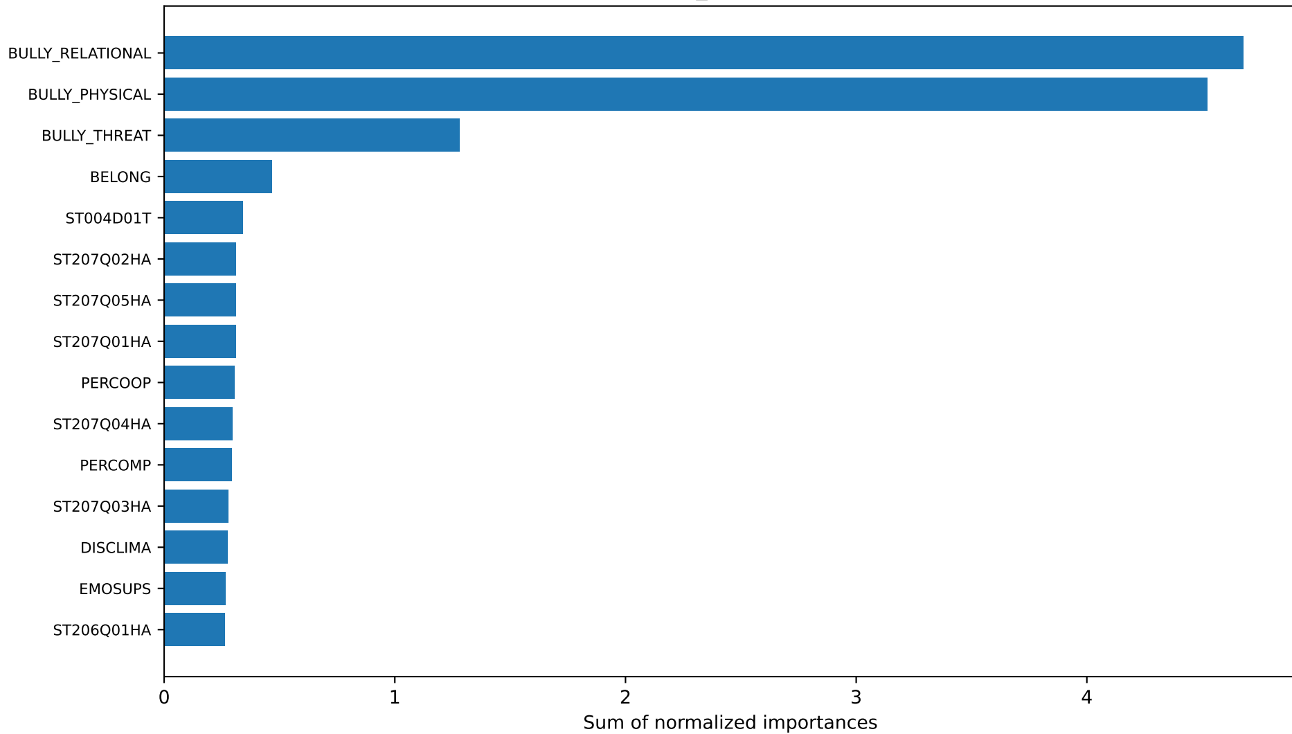
Aggregate Predictors by Cluster — BULLY_VERBAL (Full ranking, normalized) — Cluster 1
