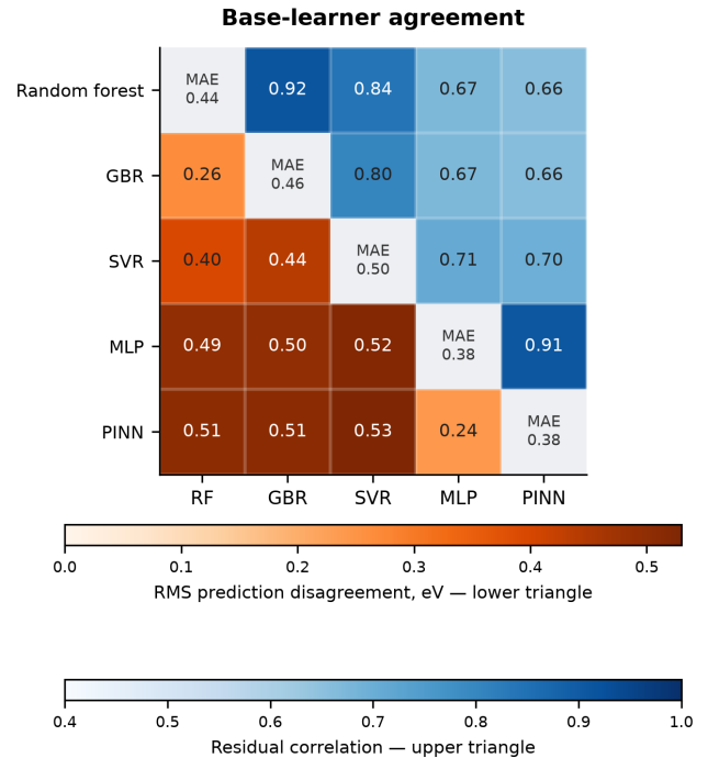
FIGURE 9. Pearson correlation between out-of-fold residuals of the base learners. Lower correlation between clusters is what makes stacking profitable.
