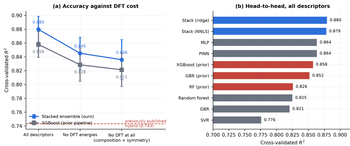
FIGURE 8. (a) Accuracy against DFT cost. Removing every DFT-derived descriptor costs 0.044 in R^2 , and the resulting model still exceeds the previously published full-descriptor hybrid. (b) Head-to-head within the full tier; red bars are the estimators specified by the prior pipeline, at their original hyperparameters, on identical folds.
