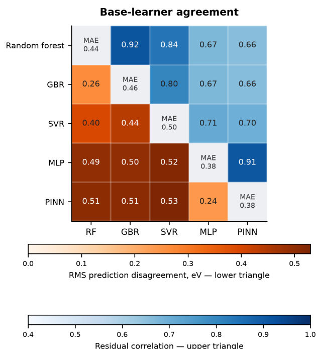
FIGURE 9. Pearson correlation between out-of-fold residuals of the base learners. Lower correlation between clusters is what makes stacking profitable.
