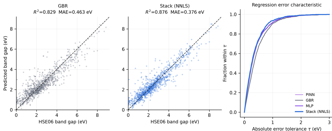
FIGURE 2. Left and centre: out-of-fold predictions against HSE06 reference values for the gradient-boosting baseline and the stacked ensemble, from a single repeat of the protocol so that each material appears once. Panel scores therefore differ slightly from the 25-estimate means in Table 3. Right: regression error characteristic curves, giving the fraction of materials predicted within a given absolute tolerance \tau .
