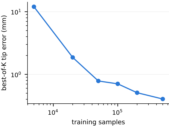
(a) accuracy vs. dataset size
