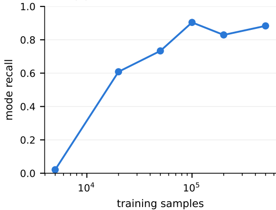
(b) mode recall vs. dataset size
