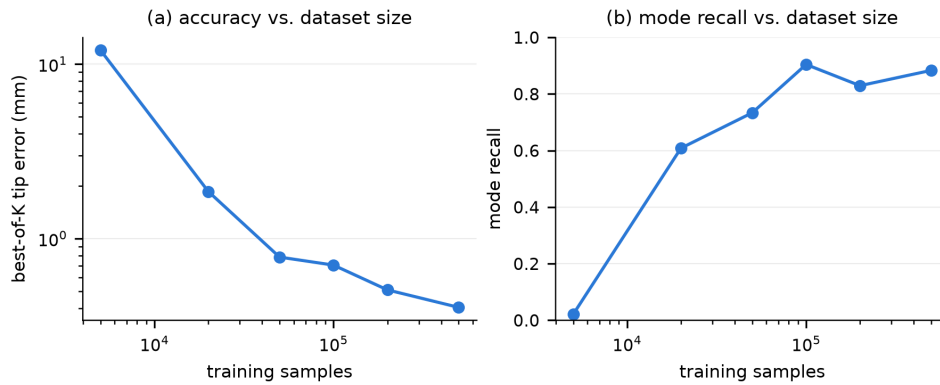
Figure 3. Single-arm dataset-size ablation on the nominal arm (single seed). (a) Best-of-K tip error and (b) mode recall vs. training-set size; both saturate by \sim 0.5 – 1 \times 10^5 samples. The amortized model reaches the 5 \times 10^5 -sample specialist’s accuracy on every in-distribution arm with the same total budget spread across the family.
