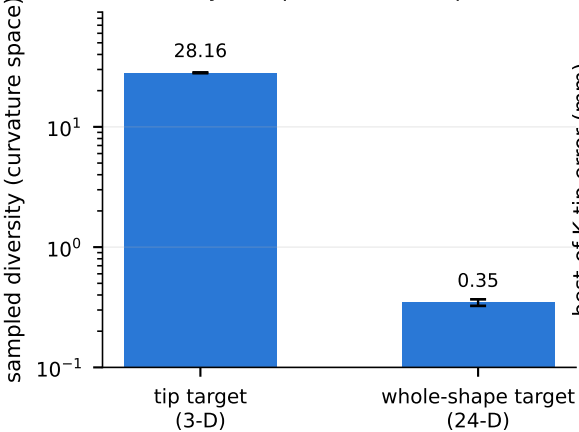
(a) redundancy collapses under shape conditioning
