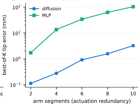
(b) advantage grows with redundancy
