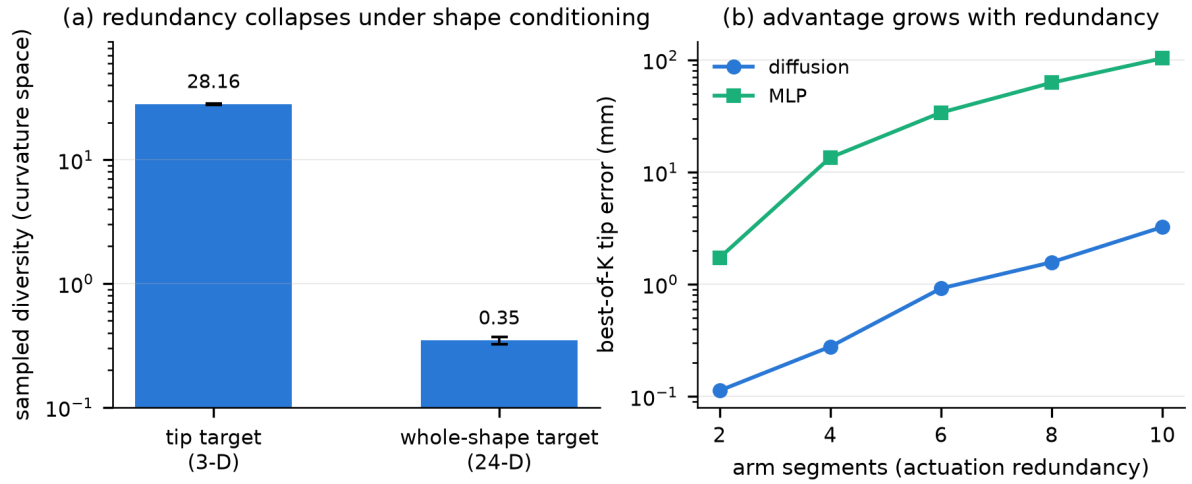
Figure 2. The diffusion advantage tracks actuation redundancy. (a) Replacing the 3-D tip target with a 24-D whole-shape target removes most of the redundancy: sampled diversity collapses \sim 80\times ( 28.16 \pm 0.22 to 0.346 \pm 0.022 ; 3 seeds). (b) Increasing the number of segments (single seed per morphology) widens the diffusion–MLP accuracy gap monotonically from two to ten segments; from eight segments on, the MLP’s obstacle-task success is 0% while diffusion’s stays \geq 99.5\% .
