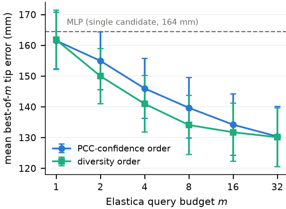
Figure 3. Candidate selection under an Elastica query budget ( n=45 targets, K=32 candidates, mean \pm SEM). A diversity-aware (farthest-point) ordering of which candidates to evaluate beats a confidence ordering; in the paired design the difference is significant at m=8 and m=16 ( t=3.34 and 3.21 , p\approx 0.002 ).
