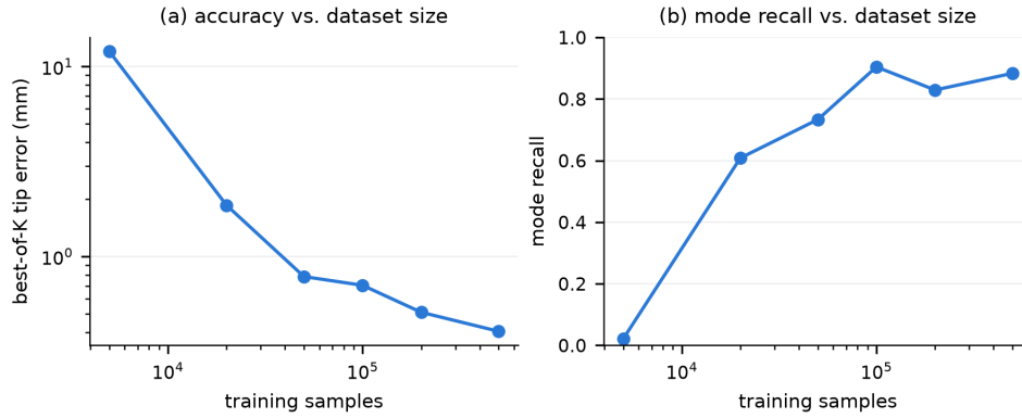
Figure 1. Single-arm dataset-size ablation on the nominal arm (single seed). (a) Best-of-K tip error and (b) mode recall vs. training-set size; both saturate by \sim 0.5\text{--}1 \times 10^5 samples. The amortized model reaches the 5 \times 10^5 -sample specialist’s accuracy on every in-distribution arm with the same total budget spread across the family.
