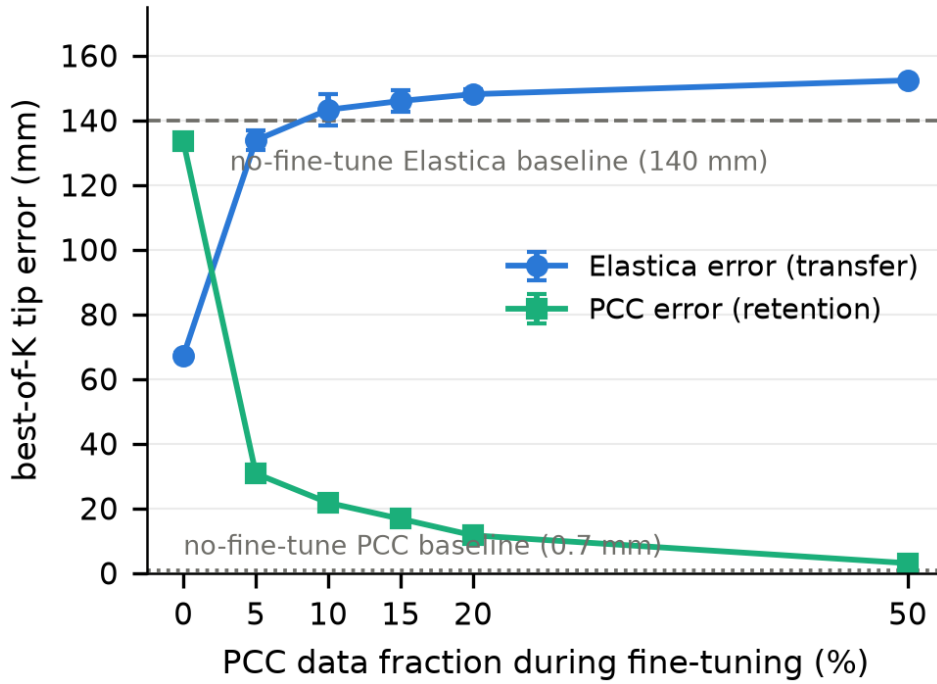
Figure 4. The retention–transfer cliff (mean \pm std, 3 seeds; six mixing ratios). Fine-tuning on 10^4 Elastica samples: retention improves smoothly as source data is mixed back in, but the transfer gain collapses almost entirely by the first grid point (5%). There is no sweet spot.
