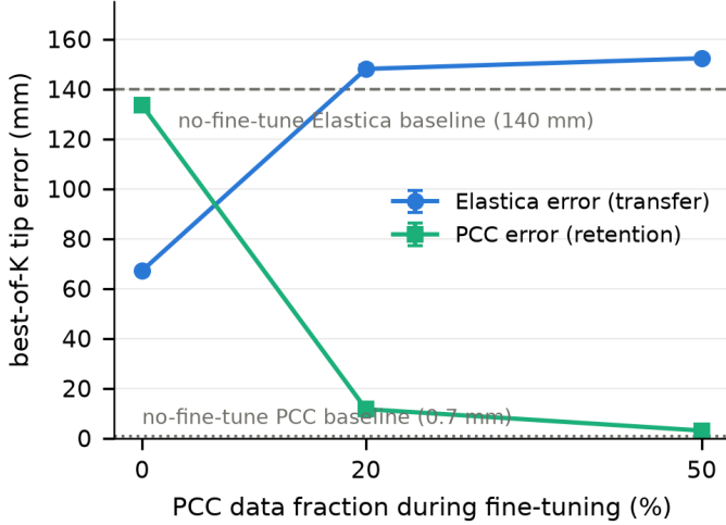
Fig. 4. The retention-transfer cliff (mean \pm std, 3 seeds). Fine-tuning the PCC-pretrained model on 10^4 Elastica samples: retention (PCC error) improves smoothly as PCC data is mixed back in, but the transfer gain collapses almost entirely at just 20% PCC data. There is no data-mixing sweet spot.
