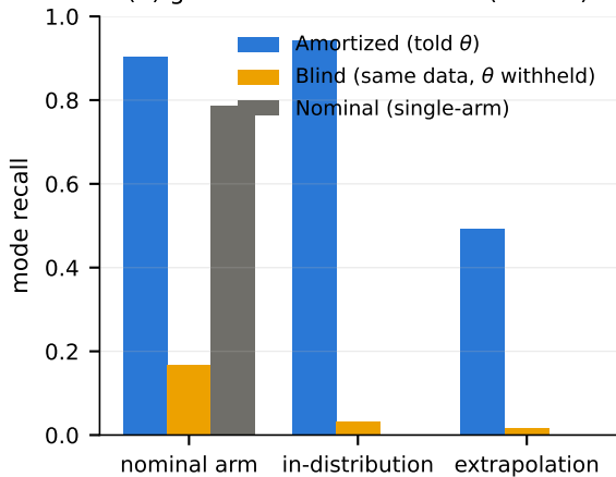
(b) ground-truth mode recall (seed 0)
