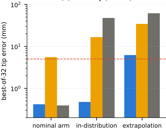
(a) accuracy (seed 0)
