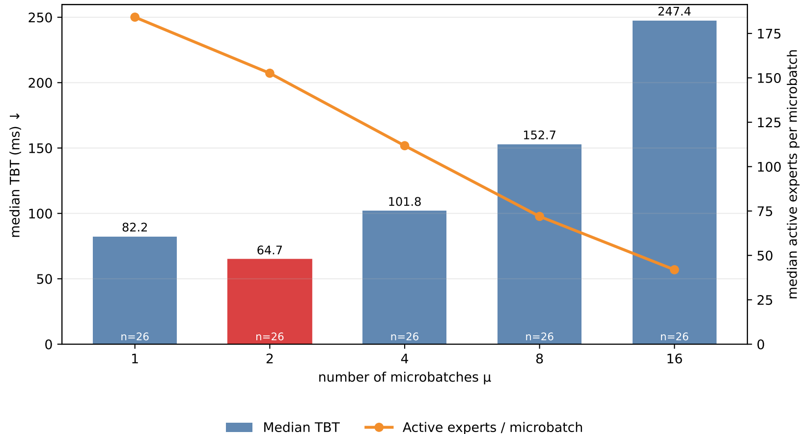
Two microbatches best balance overlap and repeated weight reads Dynamic EP, c=.98 , fixed baseline-selected budgets
