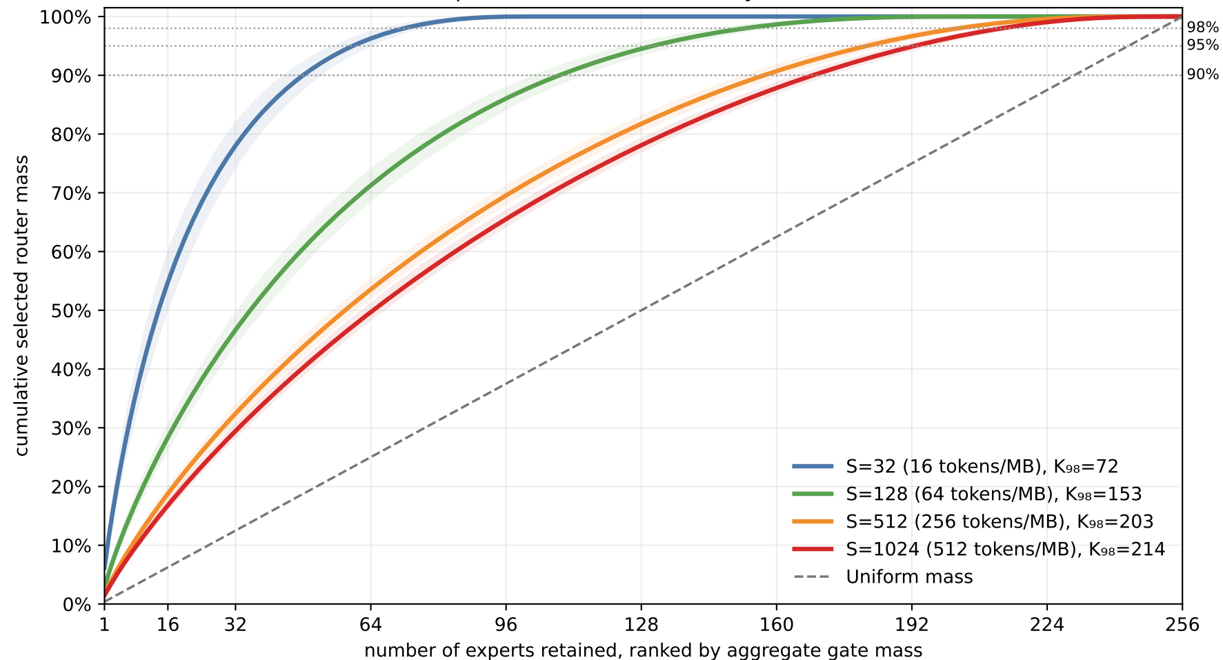
Router-mass concentration across 256 experts Mean with 10th–90th percentile bands across layers, trials, and microbatches
