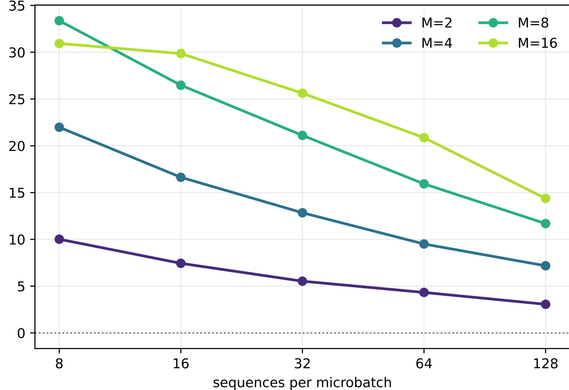
Slowest-GPU routed-token reduction
