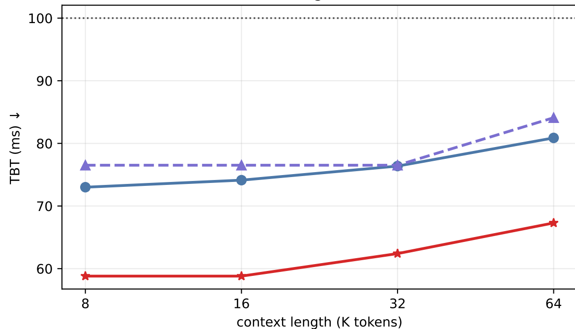
S=32, budget=8 GPUs
