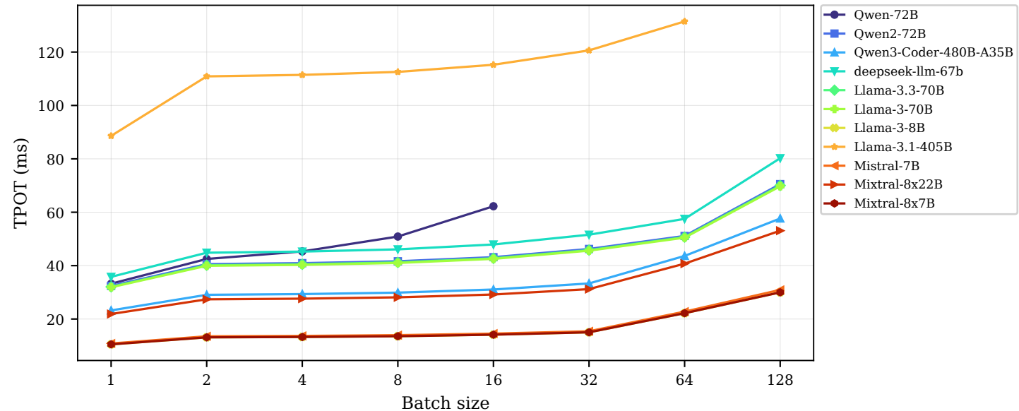
TPOT vs batch (context = 32K, SPLASH, Blackwell)
